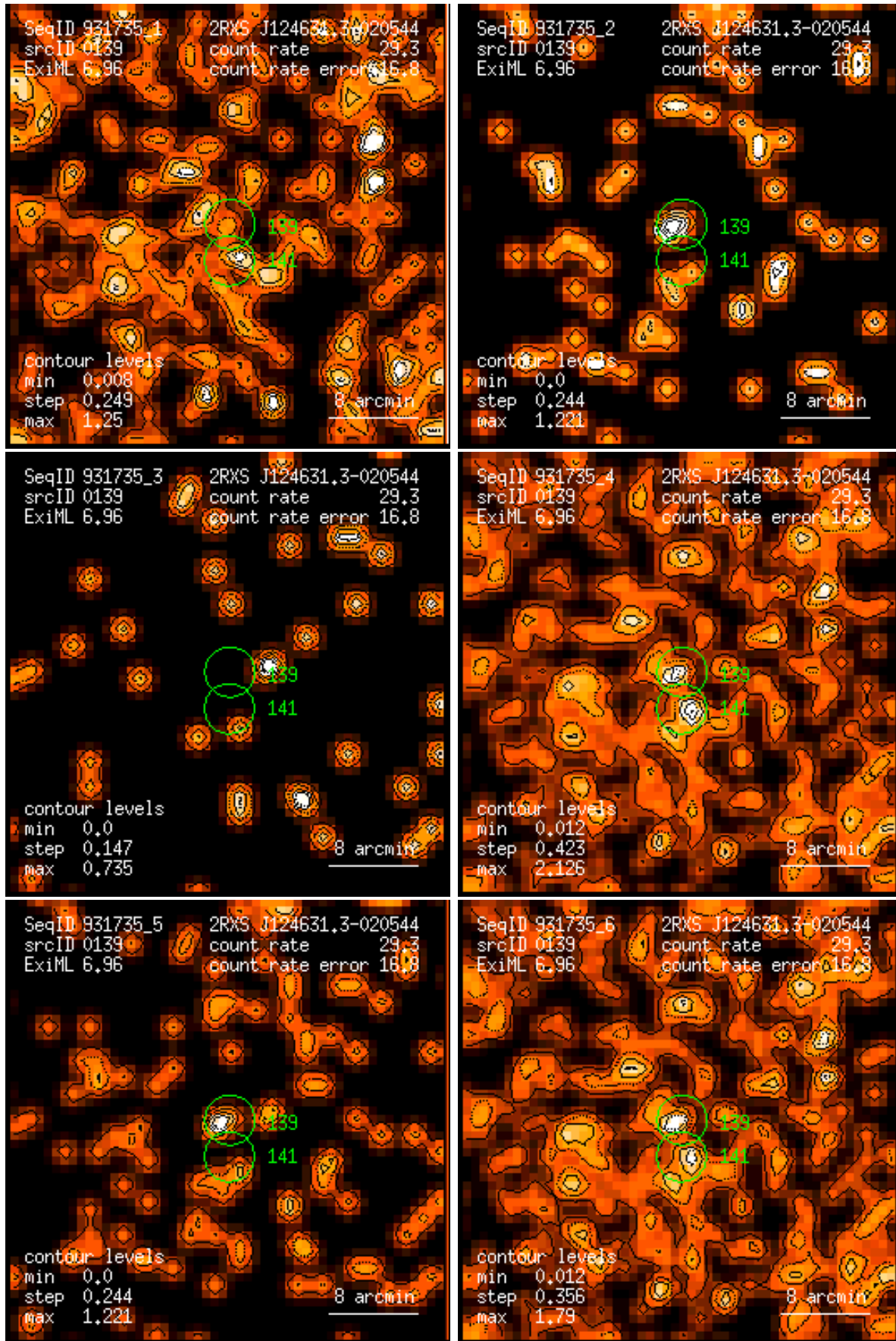
Figure 139: RASS 931735: detection 0139: band rate images, Gaussian filter: (1) PSPC channels 11 – 41, (2) 52 – 90, (3) 91 – 201, (4) 11 – 235, (5) 52 – 201, (6) 11 – 201. Broad band rates in counts/ks. Band rate contour levels in counts/ks/arcmin 2 .
