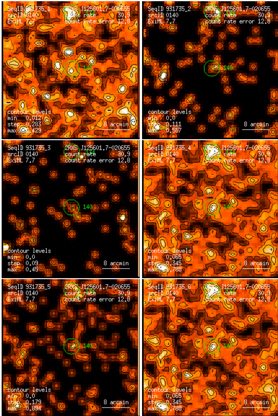
Figure 140: RASS 931735: detection 0140: band rate images, Gaussian filter: (1) PSPC channels 11 – 41, (2) 52 – 90, (3) 91 – 201, (4) 11 – 235, (5) 52 – 201, (6) 11 – 201. Broad band rates in counts/ks. Band rate contour levels in counts/ks/arcmin 2 .
