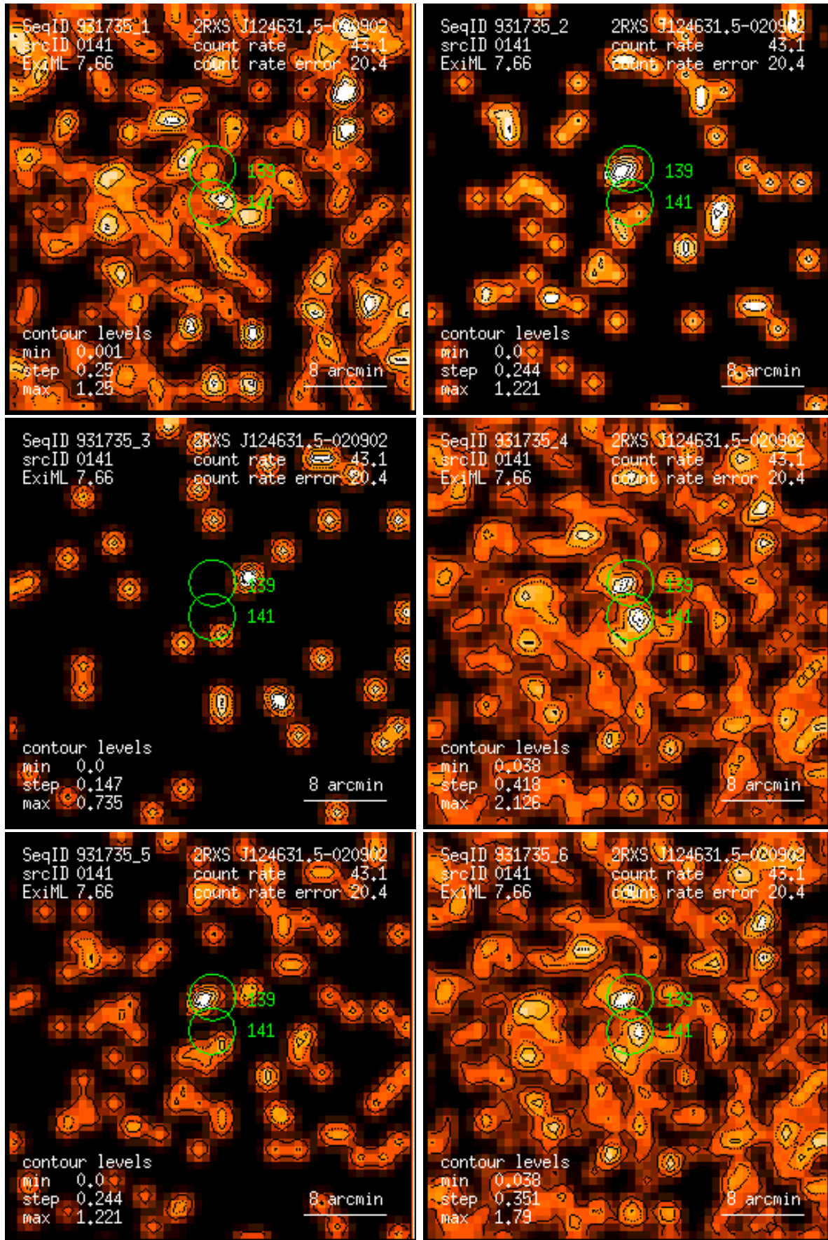
Figure 141: RASS 931735: detection 0141: band rate images, Gaussian filter: (1) PSPC channels 11 – 41, (2) 52 – 90, (3) 91 – 201, (4) 11 – 235, (5) 52 – 201, (6) 11 – 201. Broad band rates in counts/ks. Band rate contour levels in counts/ks/arcmin 2 .
