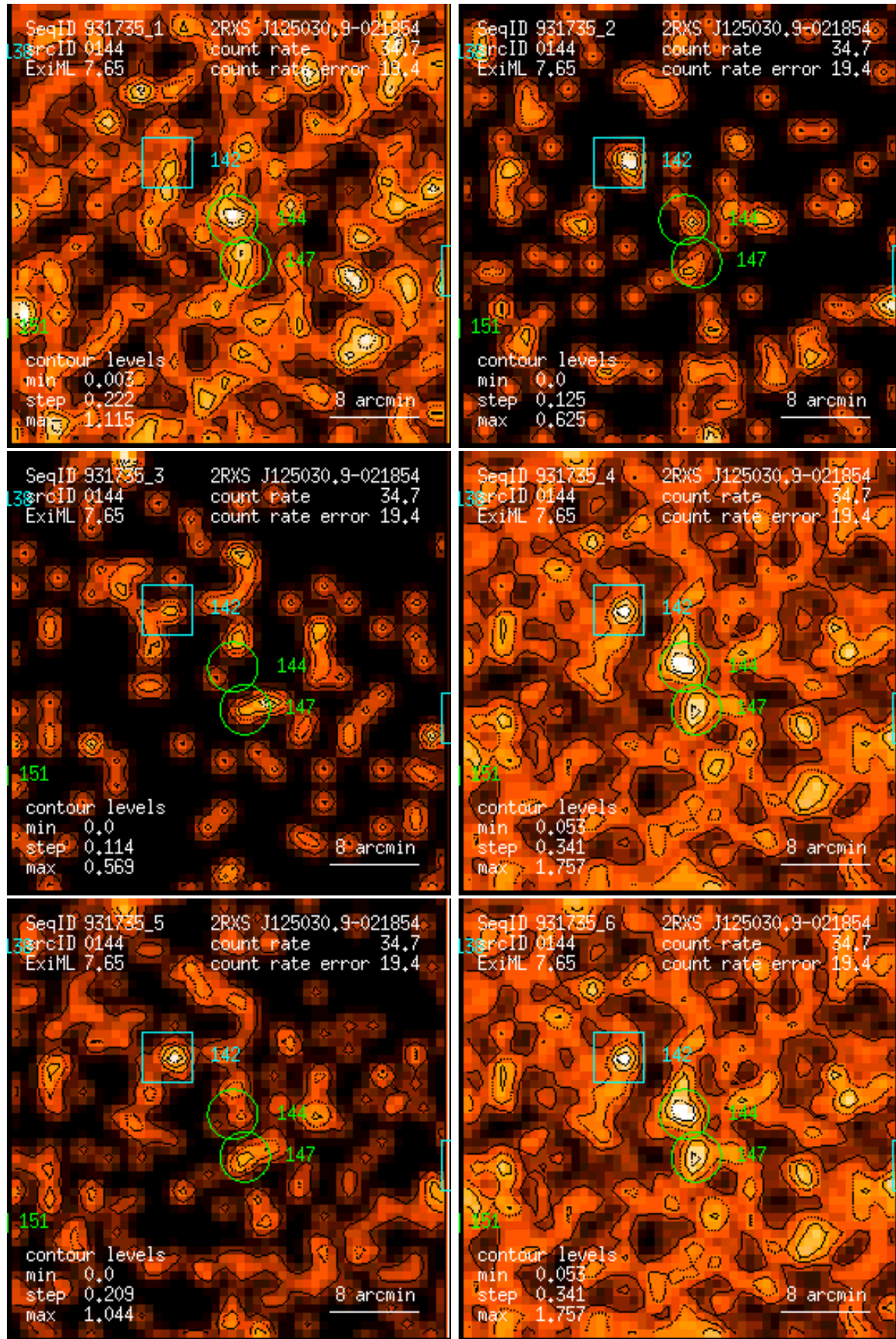
Figure 144: RASS 931735: detection 0144: band rate images, Gaussian filter: (1) PSPC channels 11 – 41, (2) 52 – 90, (3) 91 – 201, (4) 11 – 235, (5) 52 – 201, (6) 11 – 201. Broad band rates in counts/ks. Band rate contour levels in counts/ks/arcmin 2 .
