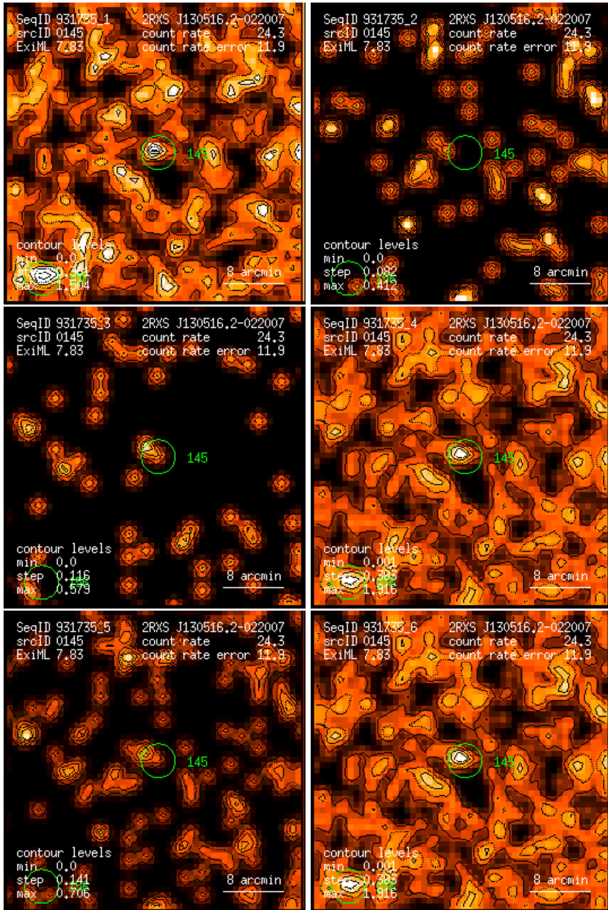
Figure 145: RASS 931735: detection 0145: band rate images, Gaussian filter: (1) PSPC channels 11 – 41, (2) 52 – 90, (3) 91 – 201, (4) 11 – 235, (5) 52 – 201, (6) 11 – 201. Broad band rates in counts/ks. Band rate contour levels in counts/ks/arcmin 2 .
