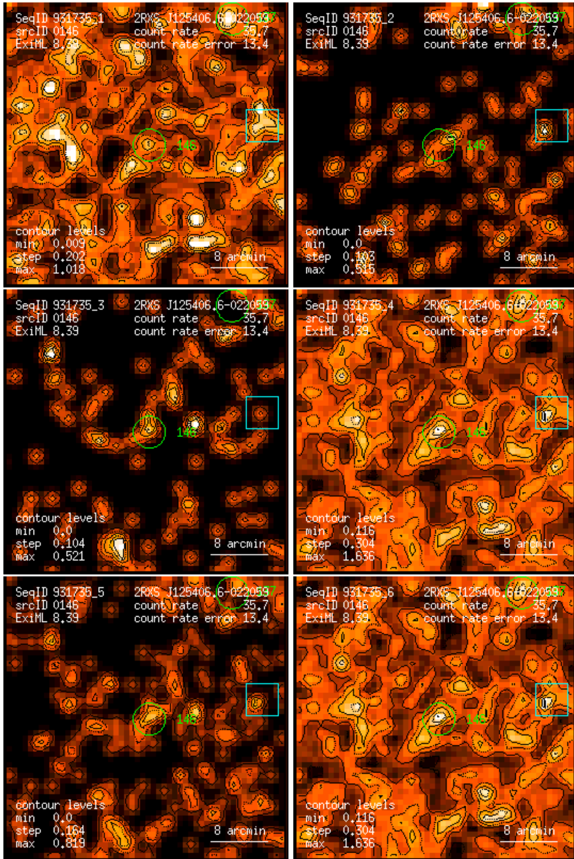
Figure 146: RASS 931735: detection 0146: band rate images, Gaussian filter: (1) PSPC channels 11 – 41, (2) 52 – 90, (3) 91 – 201, (4) 11 – 235, (5) 52 – 201, (6) 11 – 201. Broad band rates in counts/ks. Band rate contour levels in counts/ks/arcmin 2 .
