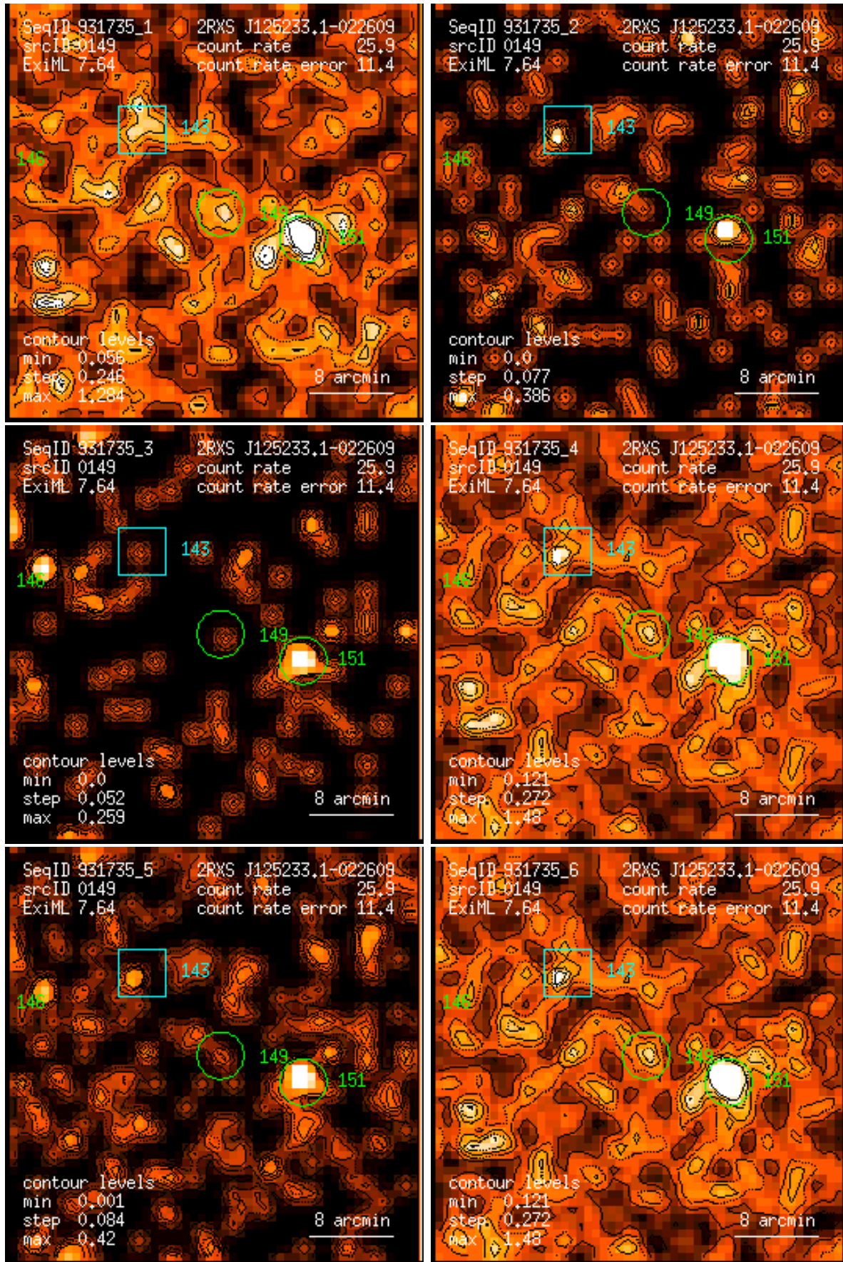
Figure 149: RASS 931735: detection 0149: band rate images, Gaussian filter: (1) PSPC channels 11 – 41, (2) 52 – 90, (3) 91 – 201, (4) 11 – 235, (5) 52 – 201, (6) 11 – 201. Broad band rates in counts/ks. Band rate contour levels in counts/ks/arcmin 2 .
