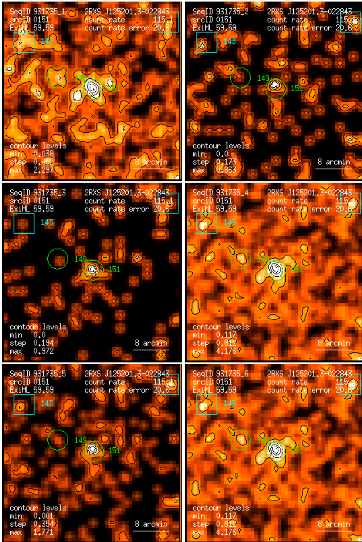
Figure 151: RASS 931735: detection 0151: band rate images, Gaussian filter: (1) PSPC channels 11 – 41, (2) 52 – 90, (3) 91 – 201, (4) 11 – 235, (5) 52 – 201, (6) 11 – 201. Broad band rates in counts/ks. Band rate contour levels in counts/ks/arcmin 2 .
