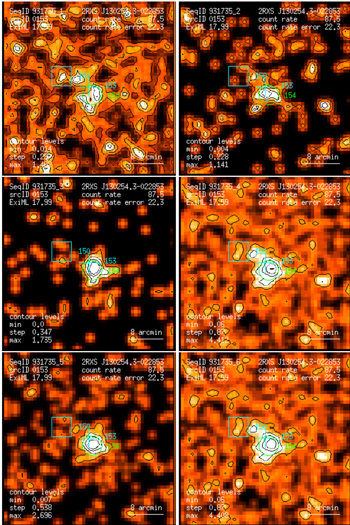
Figure 153: RASS 931735: detection 0153: band rate images, Gaussian filter: (1) PSPC channels 11 – 41, (2) 52 – 90, (3) 91 – 201, (4) 11 – 235, (5) 52 – 201, (6) 11 – 201. Broad band rates in counts/ks. Band rate contour levels in counts/ks/arcmin 2 .
