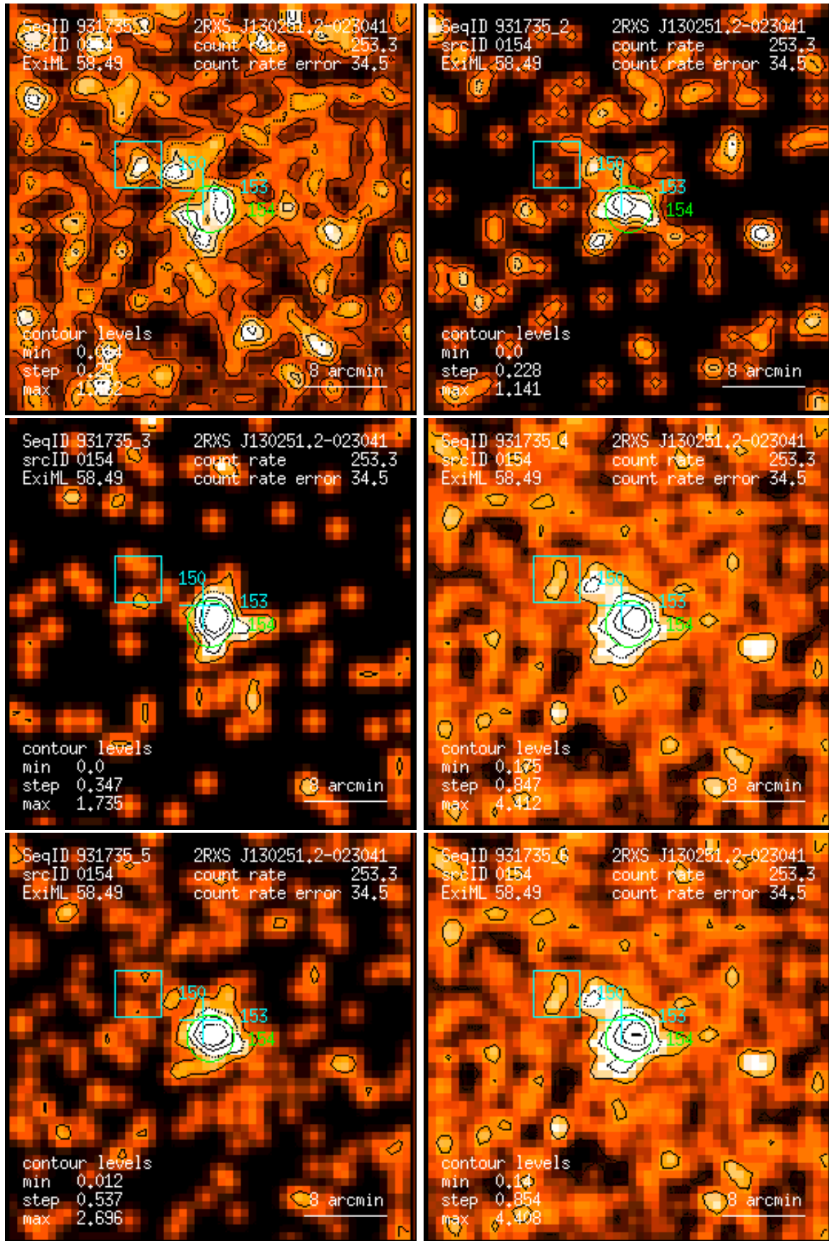
Figure 154: RASS 931735: detection 0154: band rate images, Gaussian filter: (1) PSPC channels 11 – 41, (2) 52 – 90, (3) 91 – 201, (4) 11 – 235, (5) 52 – 201, (6) 11 – 201. Broad band rates in counts/ks. Band rate contour levels in counts/ks/arcmin 2 .
