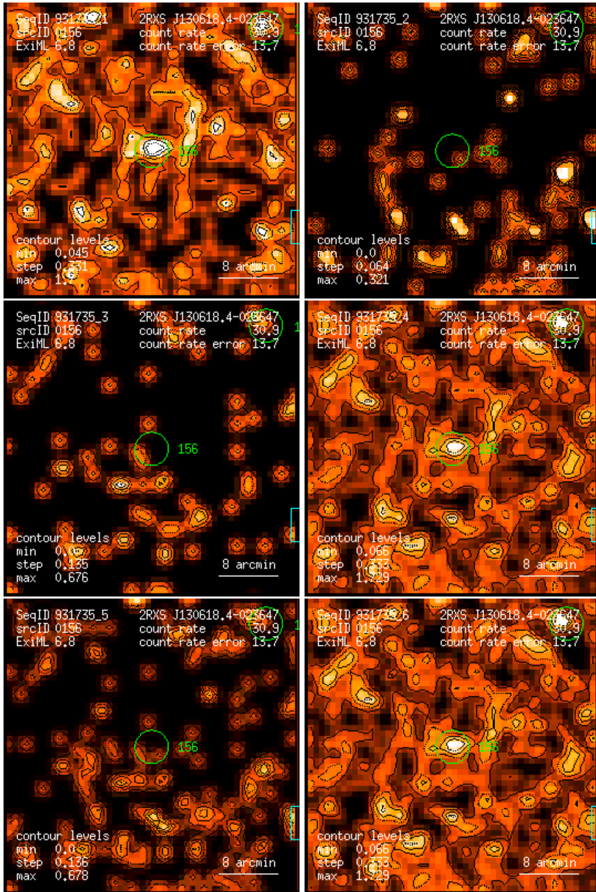
Figure 156: RASS 931735: detection 0156: band rate images, Gaussian filter: (1) PSPC channels 11 – 41, (2) 52 – 90, (3) 91 – 201, (4) 11 – 235, (5) 52 – 201, (6) 11 – 201. Broad band rates in counts/ks. Band rate contour levels in counts/ks/arcmin 2 .
