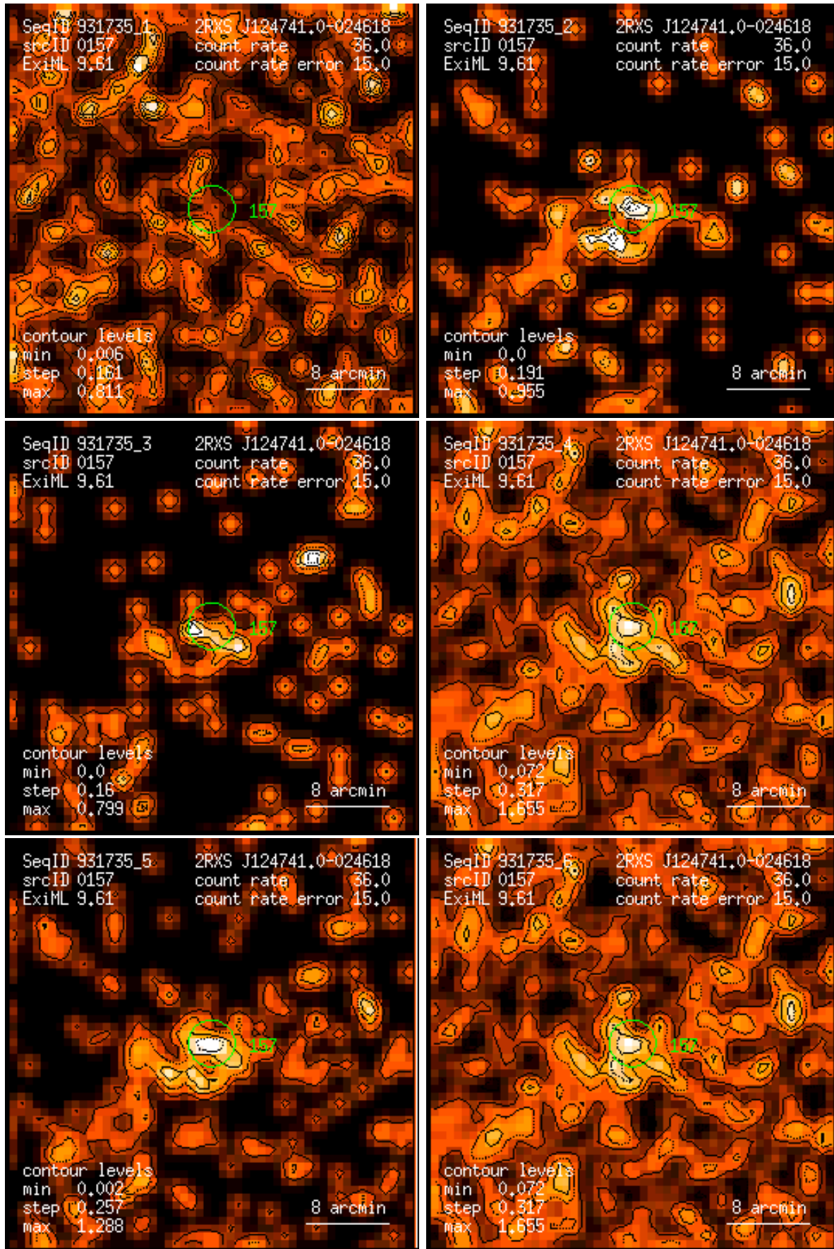
Figure 157: RASS 931735: detection 0157: band rate images, Gaussian filter: (1) PSPC channels 11 – 41, (2) 52 – 90, (3) 91 – 201, (4) 11 – 235, (5) 52 – 201, (6) 11 – 201. Broad band rates in counts/ks. Band rate contour levels in counts/ks/arcmin 2 .
