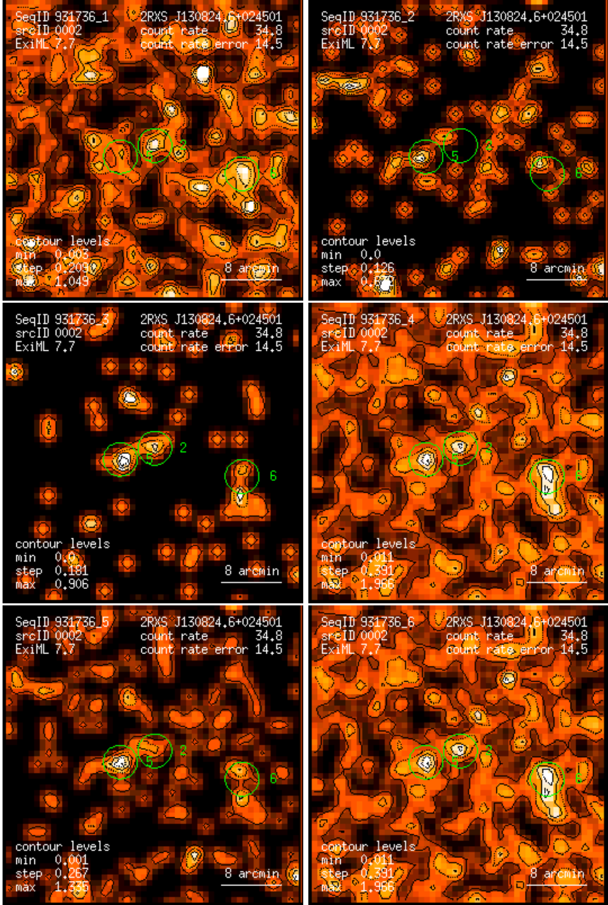
Figure 2: RASS 931736: detection 0002: band rate images, Gaussian filter: (1) PSPC channels 11 – 41, (2) 52 – 90, (3) 91 – 201, (4) 11 – 235, (5) 52 – 201, (6) 11 – 201. Broad band rates in counts/ks. Band rate contour levels in counts/ks/arcmin 2 .
