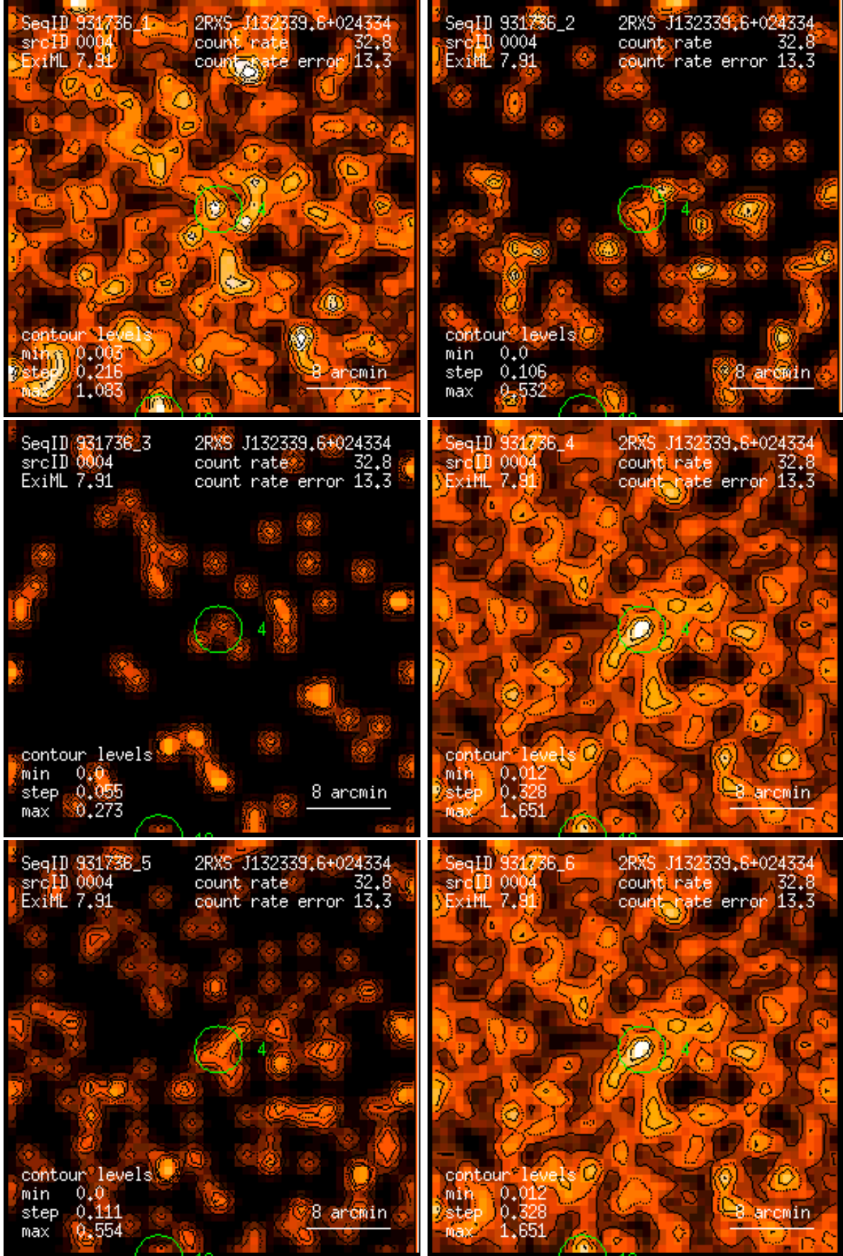
Figure 4: RASS 931736: detection 0004: band rate images, Gaussian filter: (1) PSPC channels 11 – 41, (2) 52 – 90, (3) 91 – 201, (4) 11 – 235, (5) 52 – 201, (6) 11 – 201. Broad band rates in counts/ks. Band rate contour levels in counts/ks/arcmin 2 .
