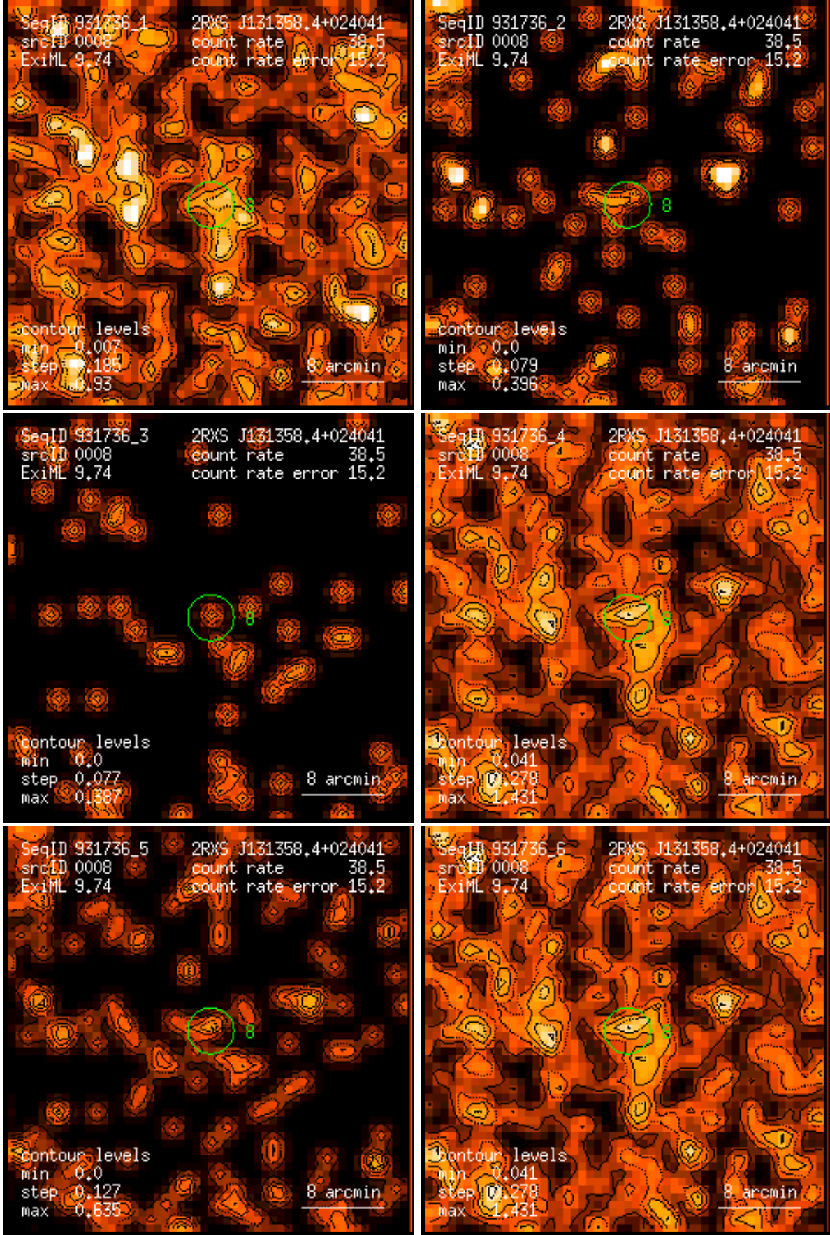
Figure 8: RASS 931736: detection 0008: band rate images, Gaussian filter: (1) PSPC channels 11 – 41, (2) 52 – 90, (3) 91 – 201, (4) 11 – 235, (5) 52 – 201, (6) 11 – 201. Broad band rates in counts/ks. Band rate contour levels in counts/ks/arcmin 2 .
