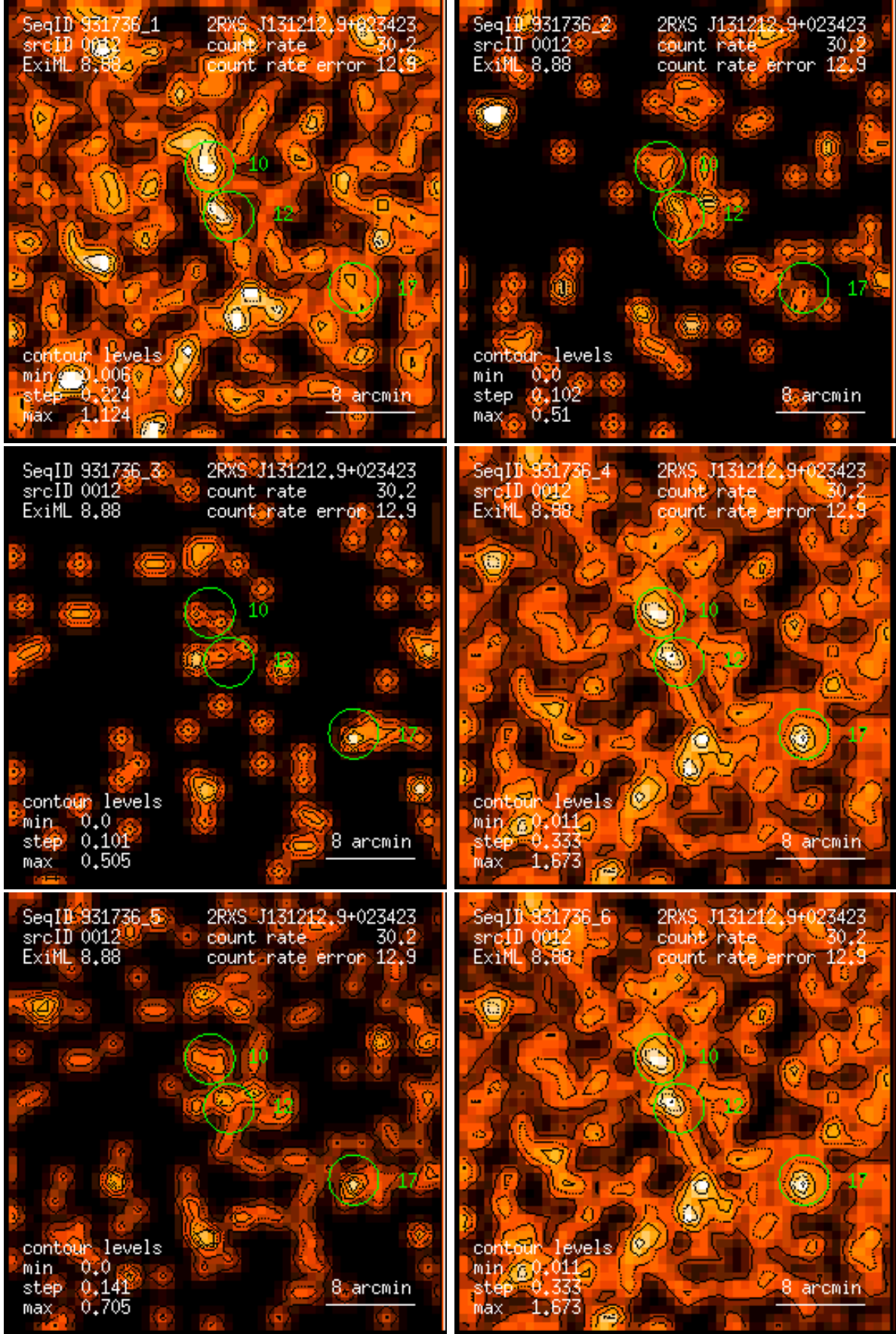
Figure 12: RASS 931736: detection 0012: band rate images, Gaussian filter: (1) PSPC channels 11 – 41, (2) 52 – 90, (3) 91 – 201, (4) 11 – 235, (5) 52 – 201, (6) 11 – 201. Broad band rates in counts/ks. Band rate contour levels in counts/ks/arcmin 2 .
