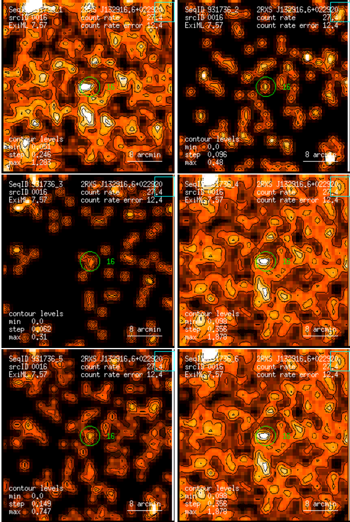
Figure 16: RASS 931736: detection 0016: band rate images, Gaussian filter: (1) PSPC channels 11 – 41, (2) 52 – 90, (3) 91 – 201, (4) 11 – 235, (5) 52 – 201, (6) 11 – 201. Broad band rates in counts/ks. Band rate contour levels in counts/ks/arcmin 2 .
