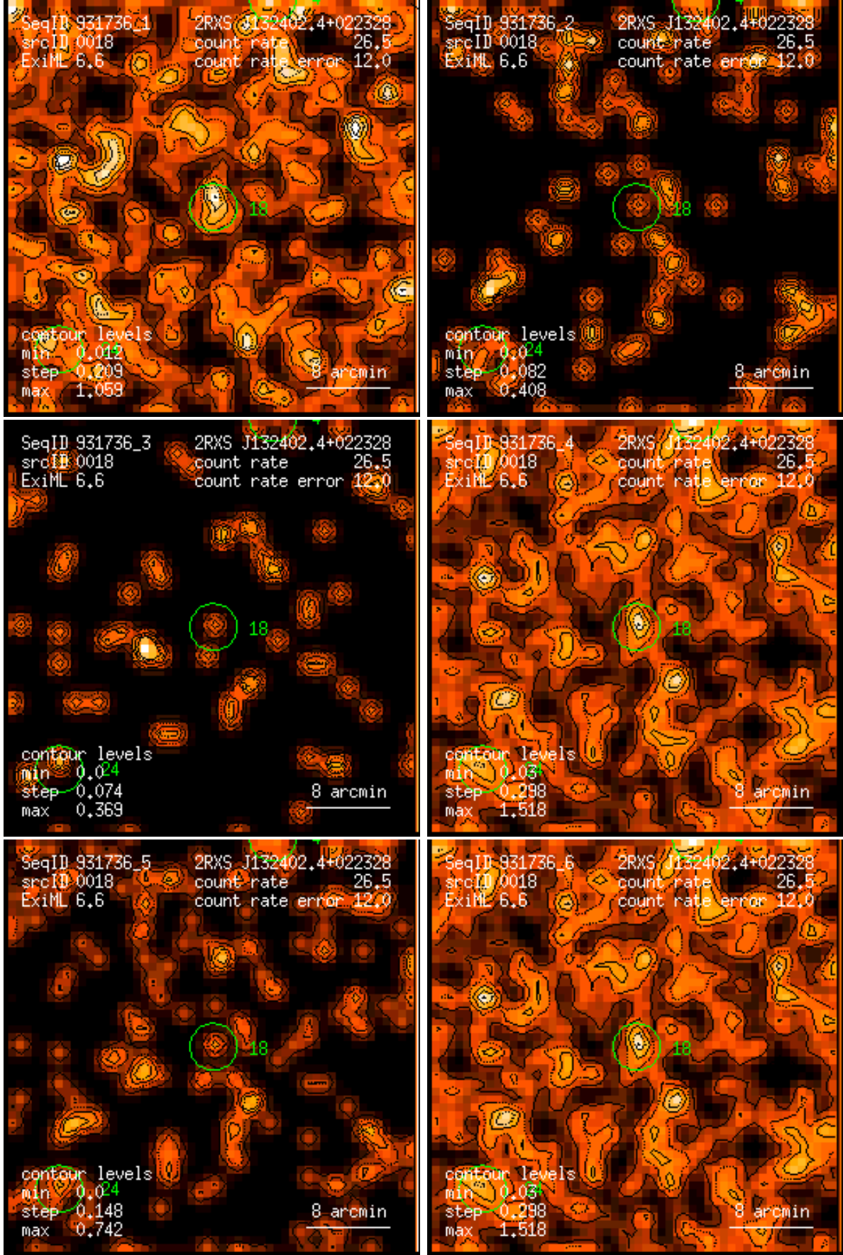
Figure 18: RASS 931736: detection 0018: band rate images, Gaussian filter: (1) PSPC channels 11 – 41, (2) 52 – 90, (3) 91 – 201, (4) 11 – 235, (5) 52 – 201, (6) 11 – 201. Broad band rates in counts/ks. Band rate contour levels in counts/ks/arcmin 2 .
