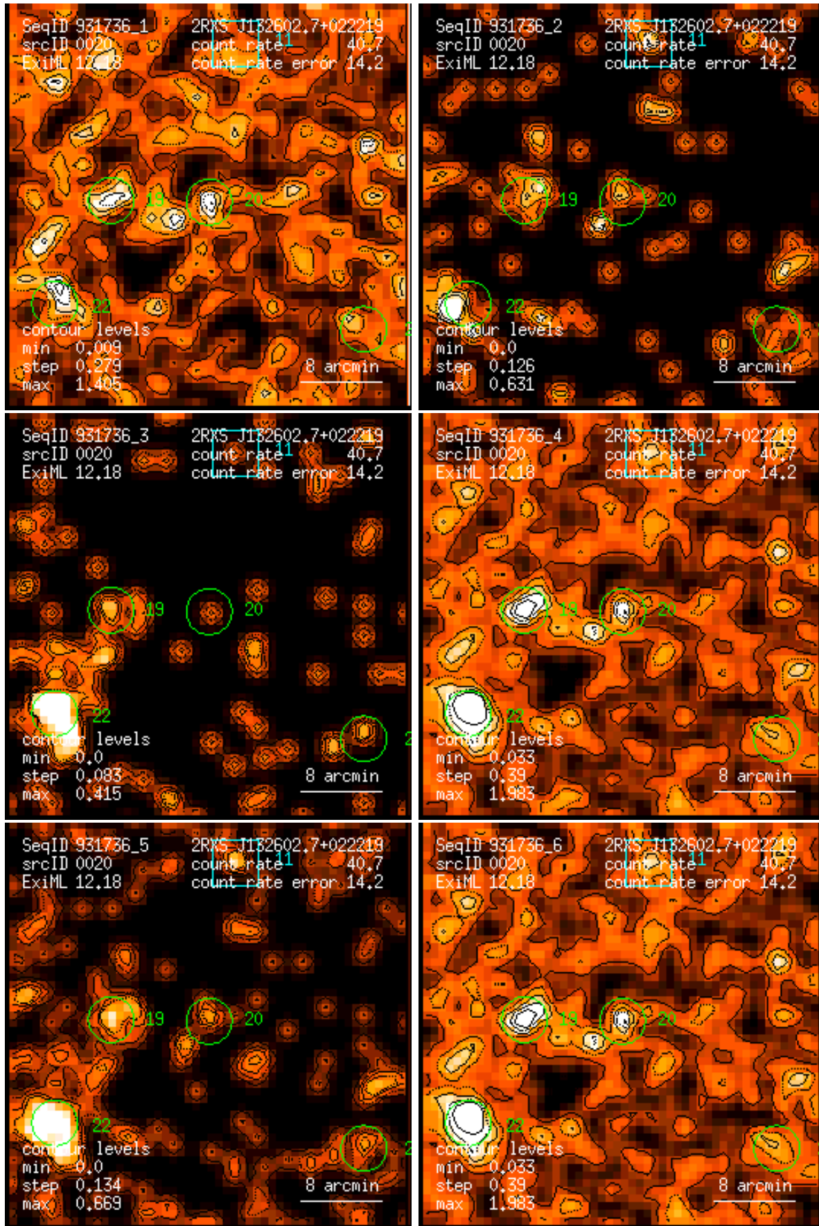
Figure 20: RASS 931736: detection 0020: band rate images, Gaussian filter: (1) PSPC channels 11 – 41, (2) 52 – 90, (3) 91 – 201, (4) 11 – 235, (5) 52 – 201, (6) 11 – 201. Broad band rates in counts/ks. Band rate contour levels in counts/ks/arcmin 2 .
