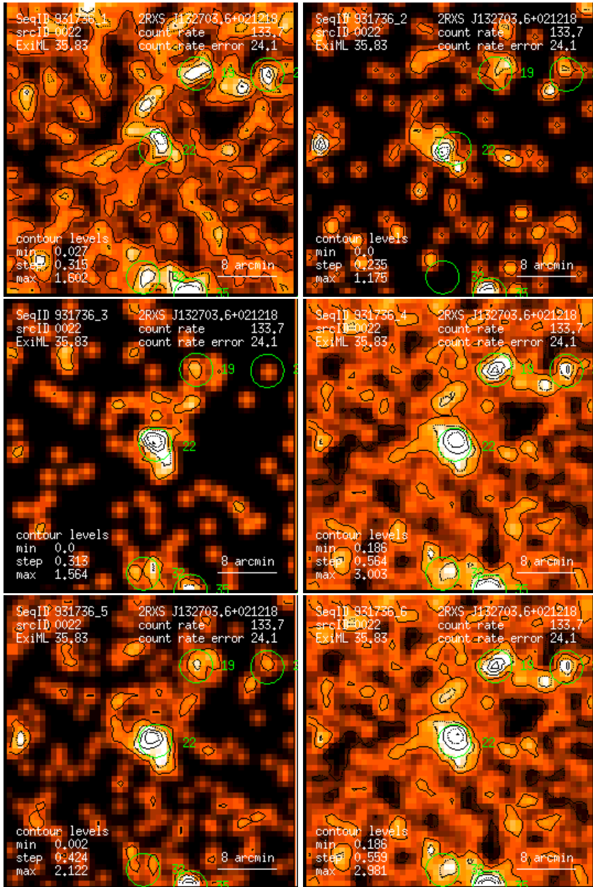
Figure 22: RASS 931736: detection 0022: band rate images, Gaussian filter: (1) PSPC channels 11 – 41, (2) 52 – 90, (3) 91 – 201, (4) 11 – 235, (5) 52 – 201, (6) 11 – 201. Broad band rates in counts/ks. Band rate contour levels in counts/ks/arcmin 2 .
