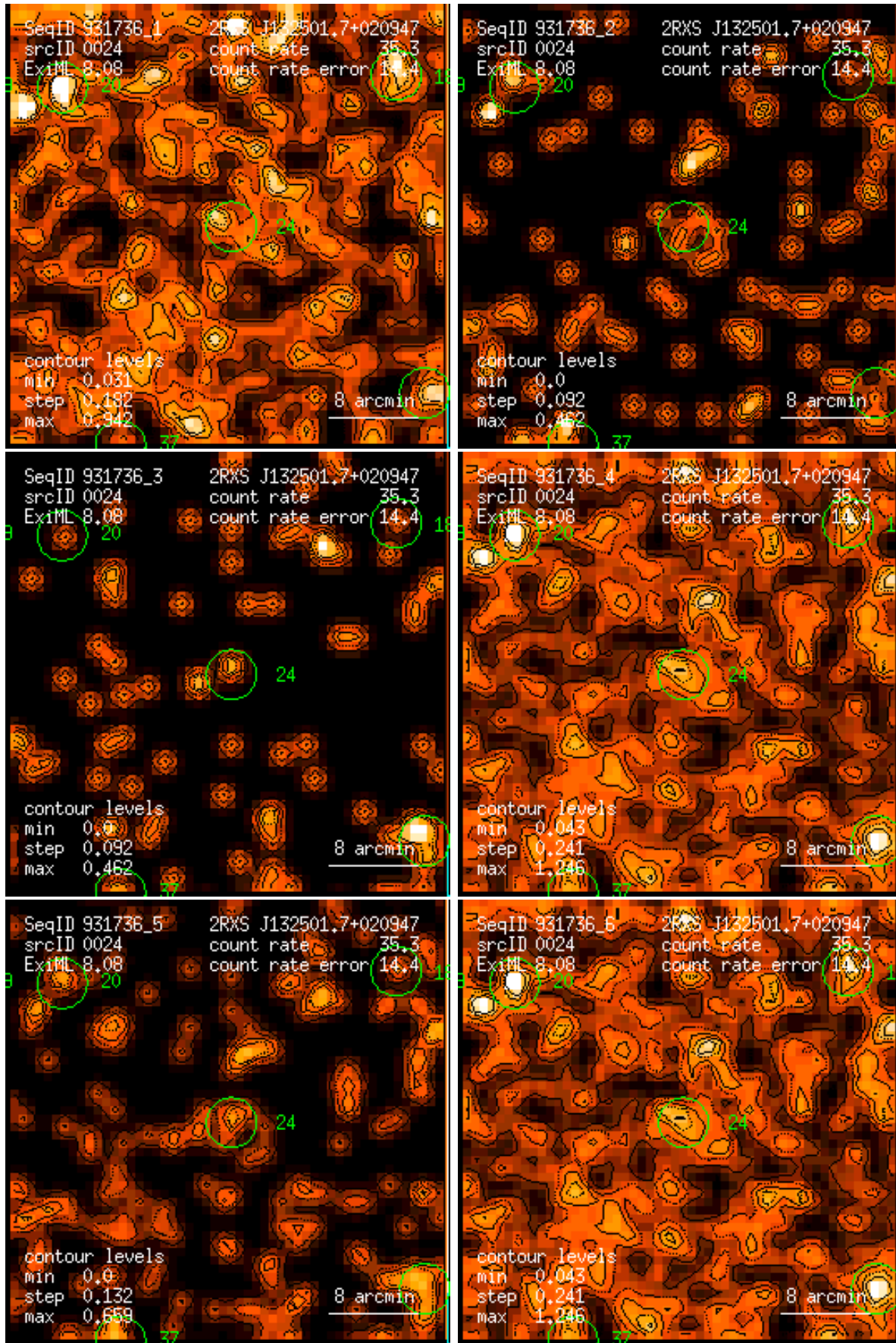
Figure 24: RASS 931736: detection 0024: band rate images, Gaussian filter: (1) PSPC channels 11 – 41, (2) 52 – 90, (3) 91 – 201, (4) 11 – 235, (5) 52 – 201, (6) 11 – 201. Broad band rates in counts/ks. Band rate contour levels in counts/ks/arcmin 2 .
