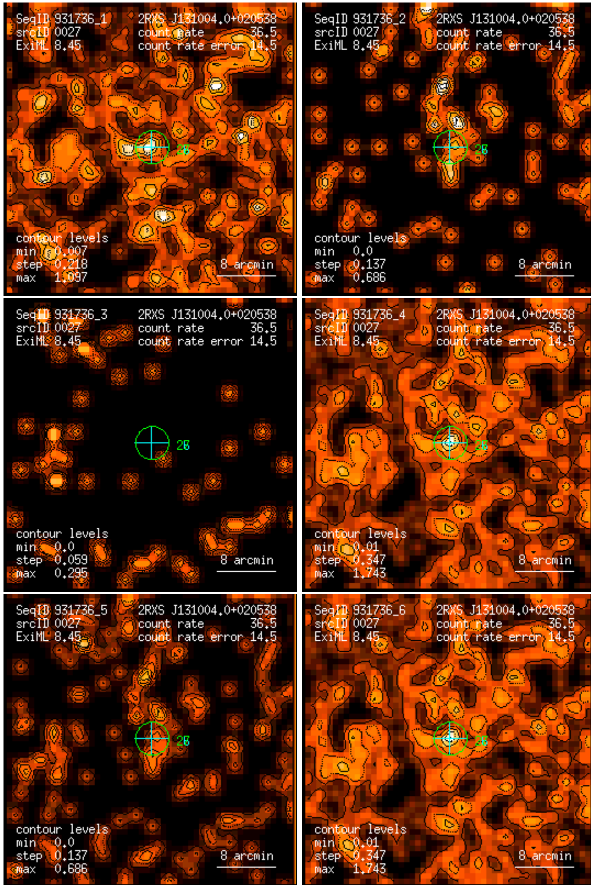
Figure 27: RASS 931736: detection 0027: band rate images, Gaussian filter: (1) PSPC channels 11 – 41, (2) 52 – 90, (3) 91 – 201, (4) 11 – 235, (5) 52 – 201, (6) 11 – 201. Broad band rates in counts/ks. Band rate contour levels in counts/ks/arcmin 2 .
