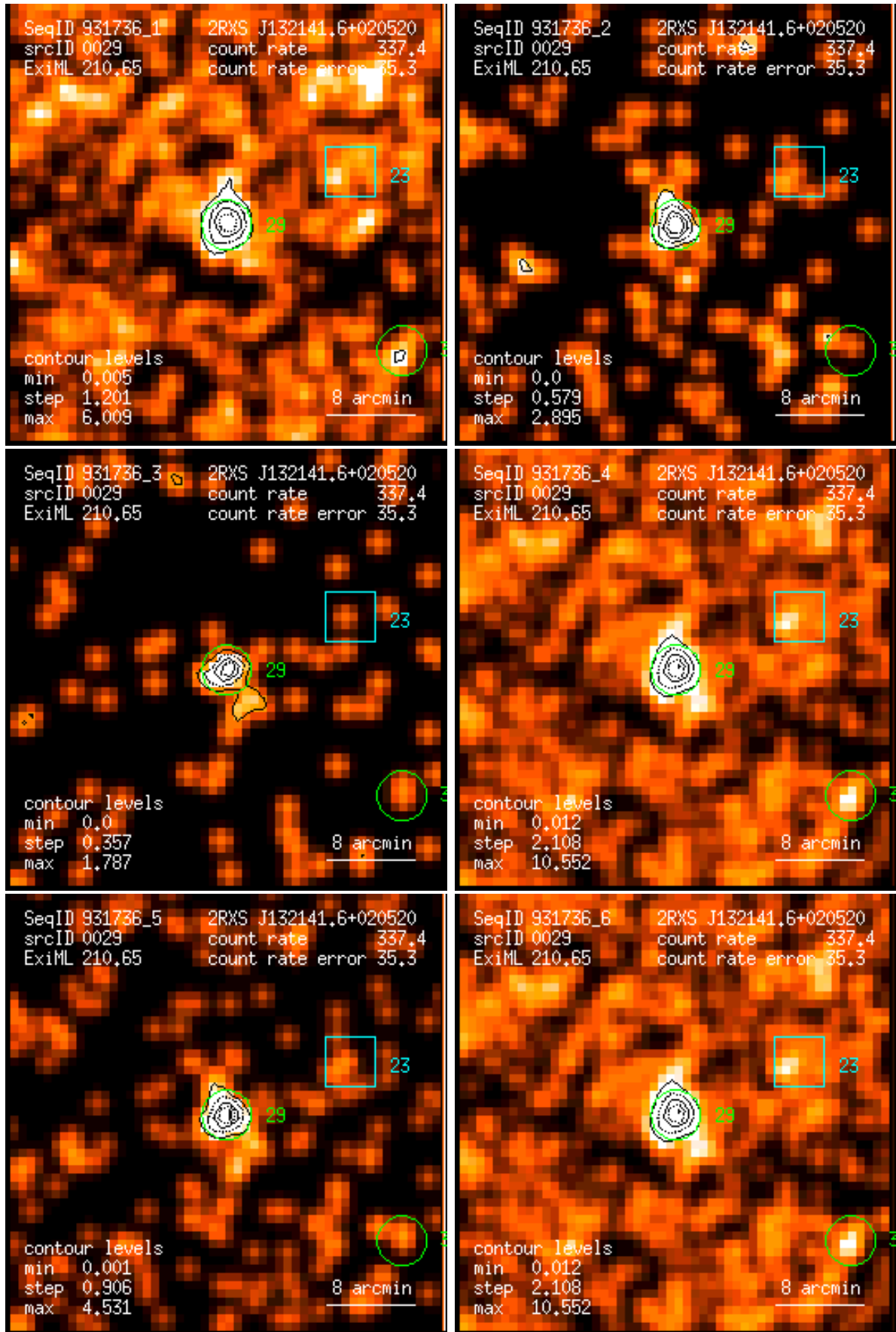
Figure 29: RASS 931736: detection 0029: band rate images, Gaussian filter: (1) PSPC channels 11 – 41, (2) 52 – 90, (3) 91 – 201, (4) 11 – 235, (5) 52 – 201, (6) 11 – 201. Broad band rates in counts/ks. Band rate contour levels in counts/ks/arcmin 2 .
