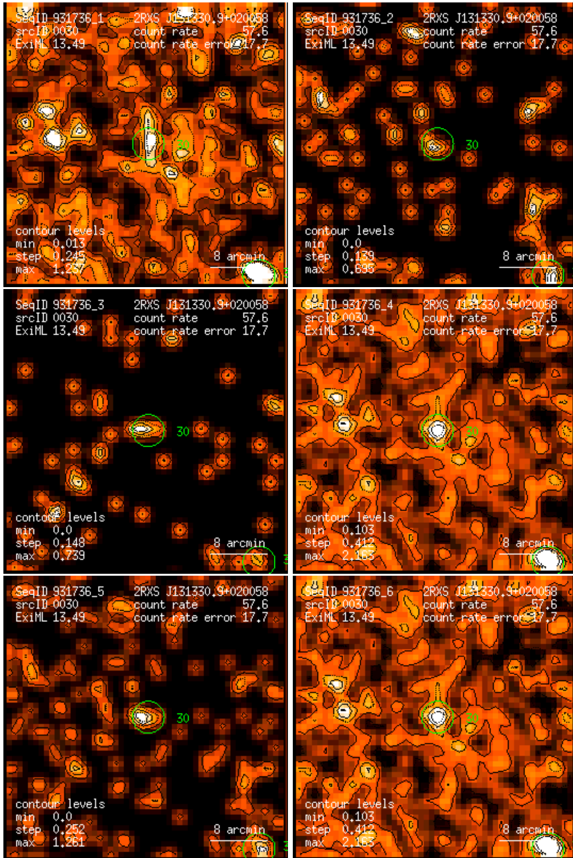
Figure 30: RASS 931736: detection 0030: band rate images, Gaussian filter: (1) PSPC channels 11 – 41, (2) 52 – 90, (3) 91 – 201, (4) 11 – 235, (5) 52 – 201, (6) 11 – 201. Broad band rates in counts/ks. Band rate contour levels in counts/ks/arcmin 2 .
