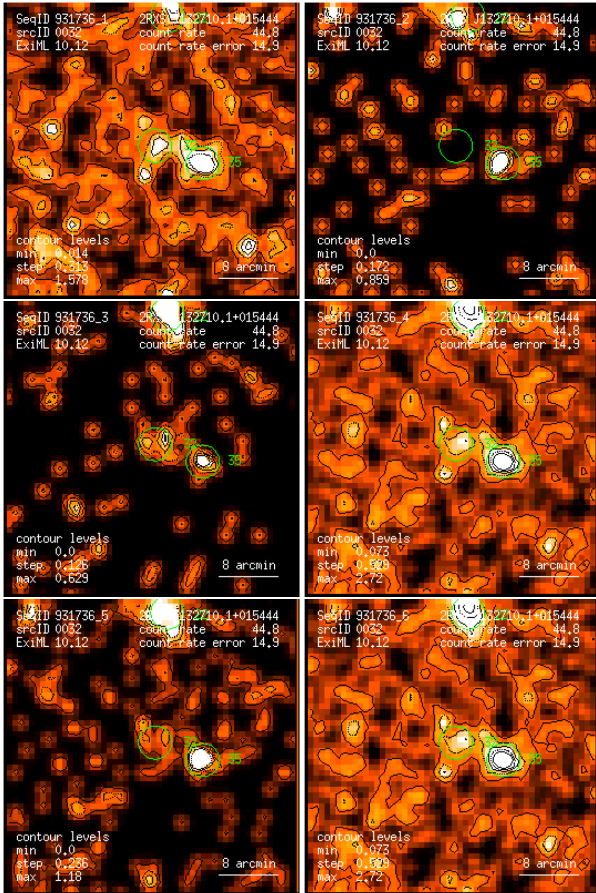
Figure 32: RASS 931736: detection 0032: band rate images, Gaussian filter: (1) PSPC channels 11 – 41, (2) 52 – 90, (3) 91 – 201, (4) 11 – 235, (5) 52 – 201, (6) 11 – 201. Broad band rates in counts/ks. Band rate contour levels in counts/ks/arcmin 2 .
