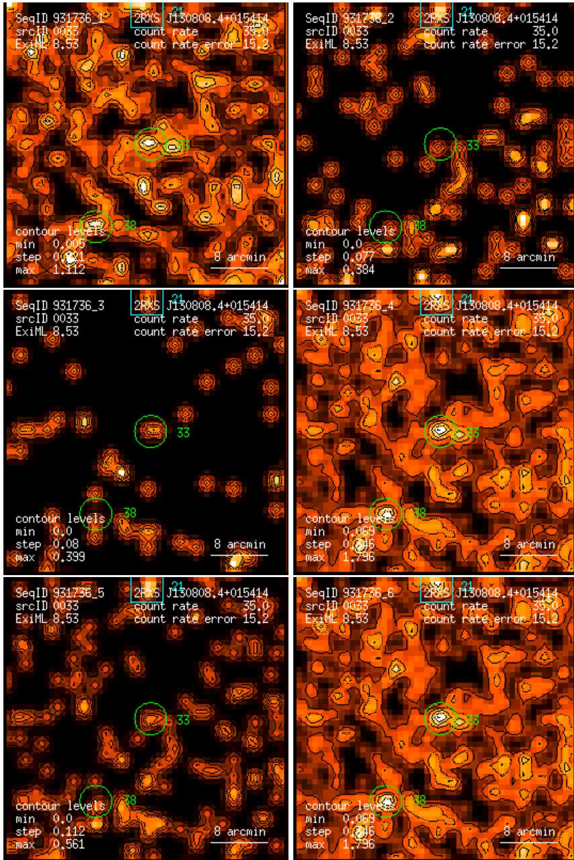
Figure 33: RASS 931736: detection 0033: band rate images, Gaussian filter: (1) PSPC channels 11 – 41, (2) 52 – 90, (3) 91 – 201, (4) 11 – 235, (5) 52 – 201, (6) 11 – 201. Broad band rates in counts/ks. Band rate contour levels in counts/ks/arcmin 2 .
