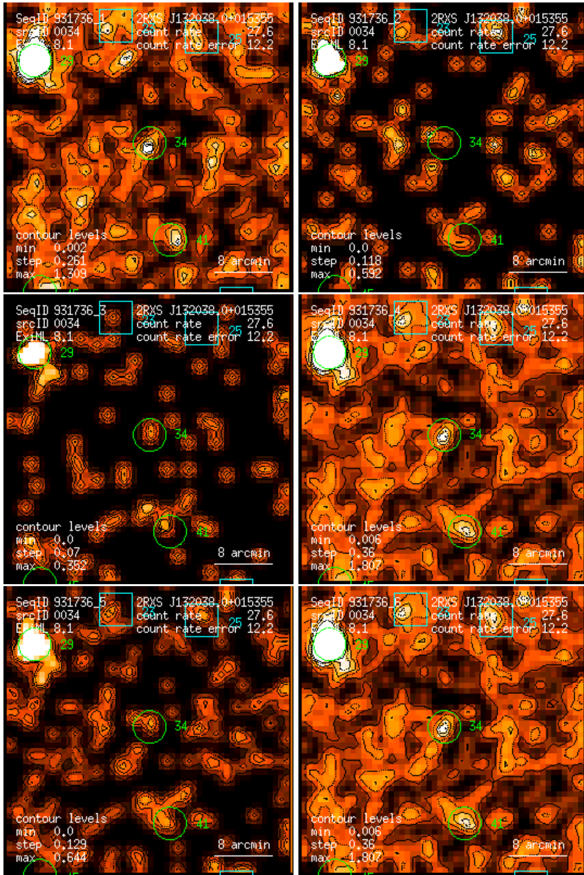
Figure 34: RASS 931736: detection 0034: band rate images, Gaussian filter: (1) PSPC channels 11 – 41, (2) 52 – 90, (3) 91 – 201, (4) 11 – 235, (5) 52 – 201, (6) 11 – 201. Broad band rates in counts/ks. Band rate contour levels in counts/ks/arcmin 2 .
