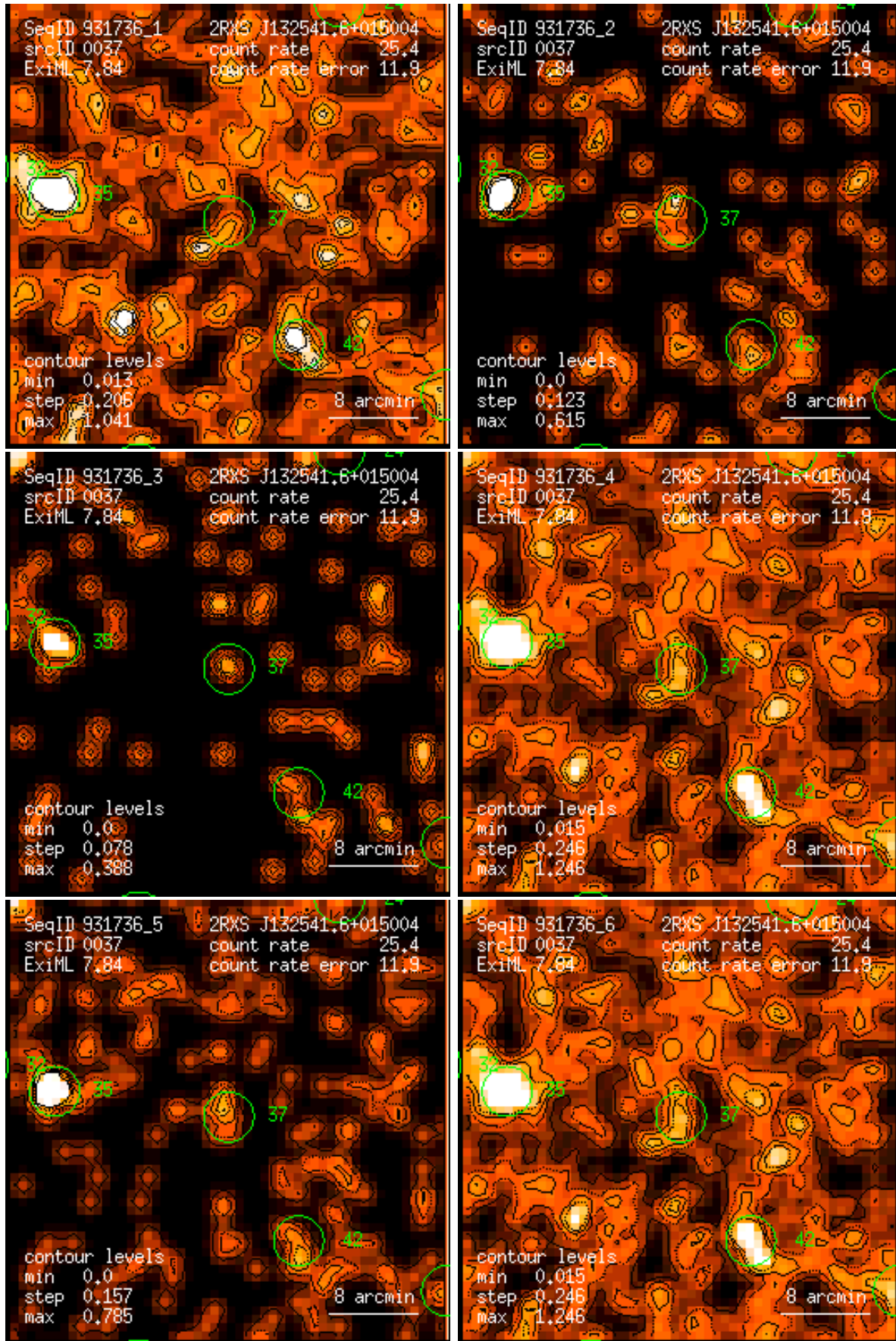
Figure 37: RASS 931736: detection 0037: band rate images, Gaussian filter: (1) PSPC channels 11 – 41, (2) 52 – 90, (3) 91 – 201, (4) 11 – 235, (5) 52 – 201, (6) 11 – 201. Broad band rates in counts/ks. Band rate contour levels in counts/ks/arcmin 2 .
