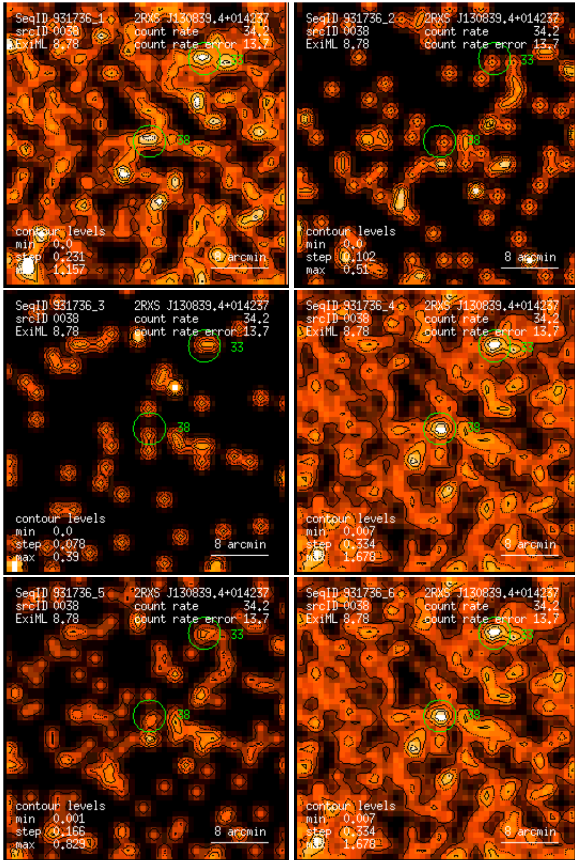
Figure 38: RASS 931736: detection 0038: band rate images, Gaussian filter: (1) PSPC channels 11 – 41, (2) 52 – 90, (3) 91 – 201, (4) 11 – 235, (5) 52 – 201, (6) 11 – 201. Broad band rates in counts/ks. Band rate contour levels in counts/ks/arcmin 2 .
