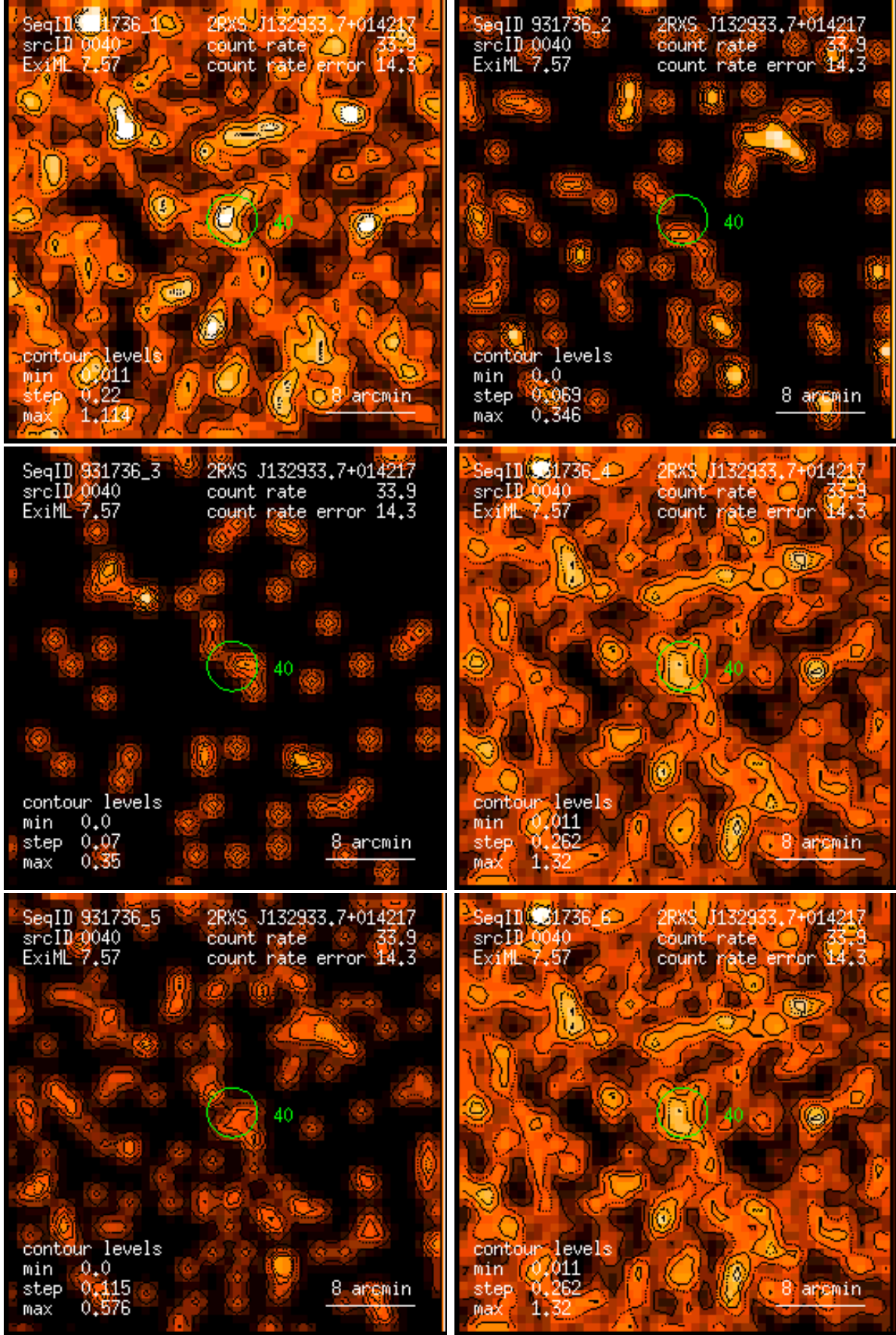
Figure 40: RASS 931736: detection 0040: band rate images, Gaussian filter: (1) PSPC channels 11 – 41, (2) 52 – 90, (3) 91 – 201, (4) 11 – 235, (5) 52 – 201, (6) 11 – 201. Broad band rates in counts/ks. Band rate contour levels in counts/ks/arcmin 2 .
