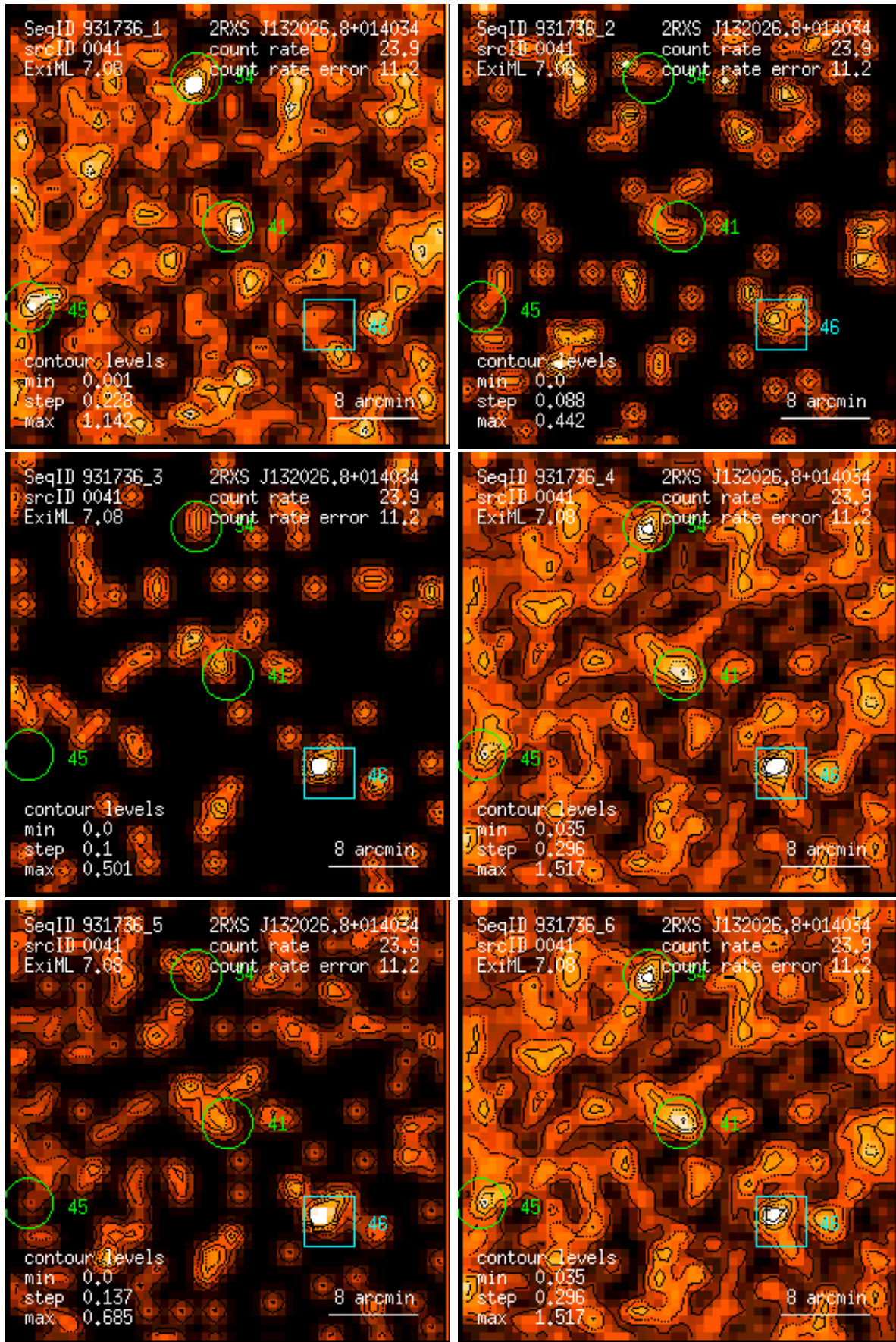
Figure 41: RASS 931736: detection 0041: band rate images, Gaussian filter: (1) PSPC channels 11 – 41, (2) 52 – 90, (3) 91 – 201, (4) 11 – 235, (5) 52 – 201, (6) 11 – 201. Broad band rates in counts/ks. Band rate contour levels in counts/ks/arcmin 2 .
