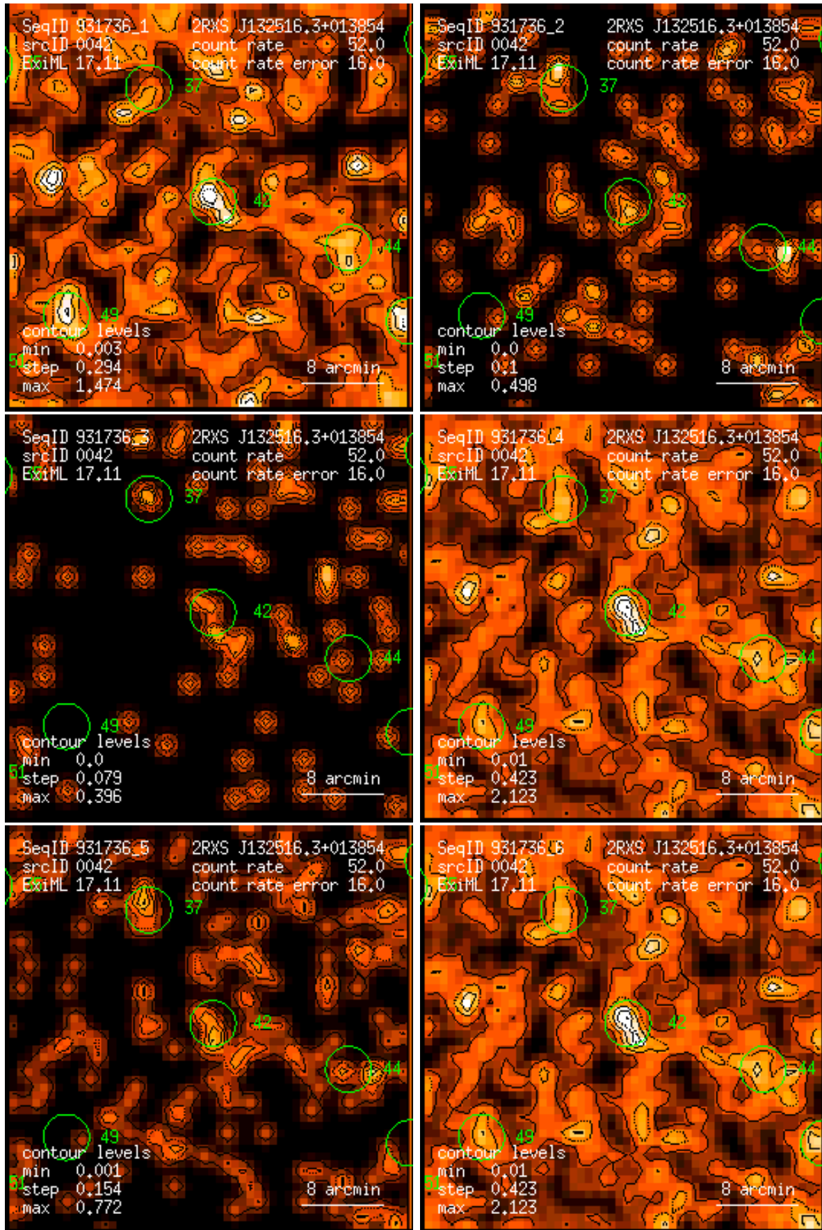
Figure 42: RASS 931736: detection 0042: band rate images, Gaussian filter: (1) PSPC channels 11 – 41, (2) 52 – 90, (3) 91 – 201, (4) 11 – 235, (5) 52 – 201, (6) 11 – 201. Broad band rates in counts/ks. Band rate contour levels in counts/ks/arcmin 2 .
