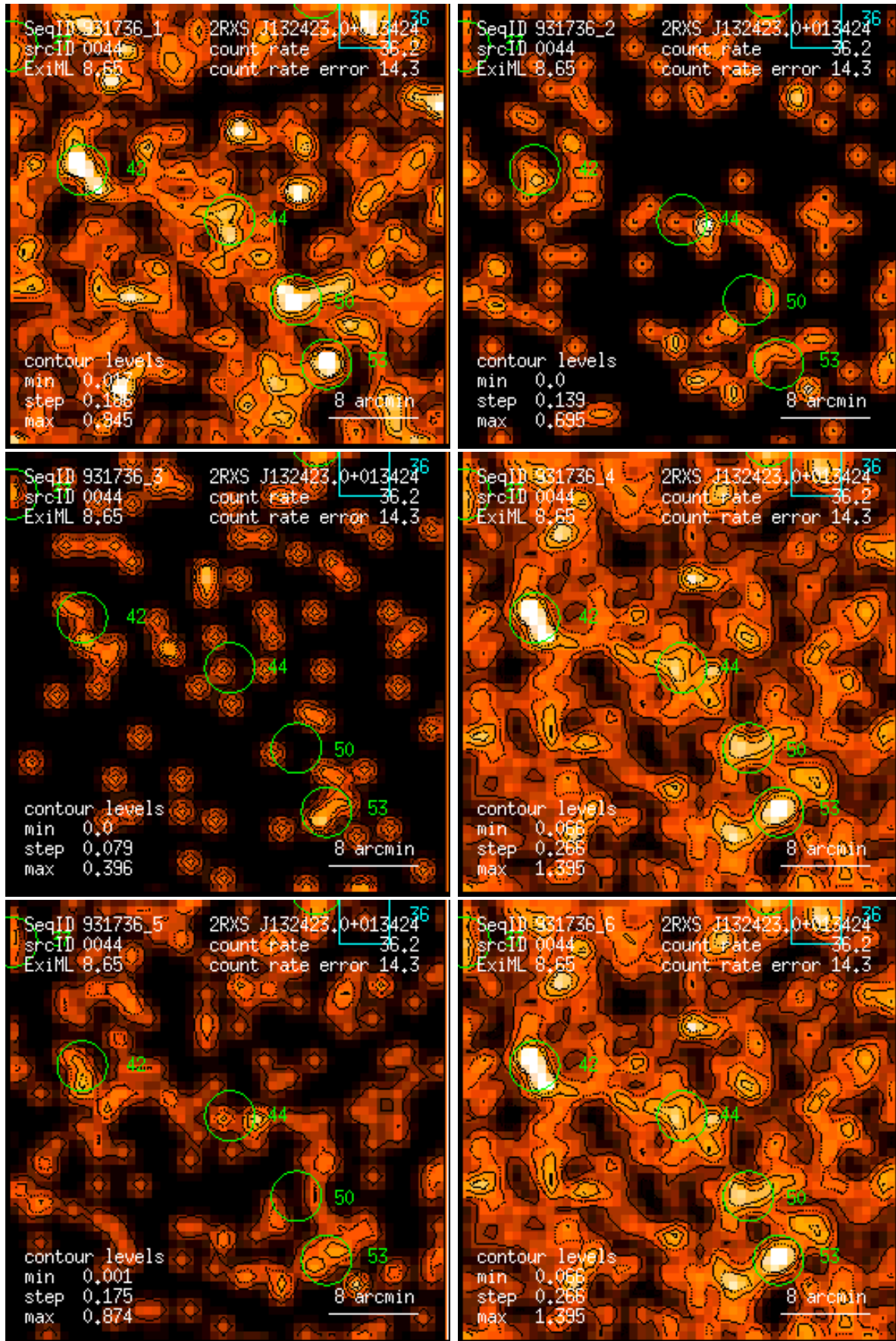
Figure 44: RASS 931736: detection 0044: band rate images, Gaussian filter: (1) PSPC channels 11 – 41, (2) 52 – 90, (3) 91 – 201, (4) 11 – 235, (5) 52 – 201, (6) 11 – 201. Broad band rates in counts/ks. Band rate contour levels in counts/ks/arcmin 2 .
