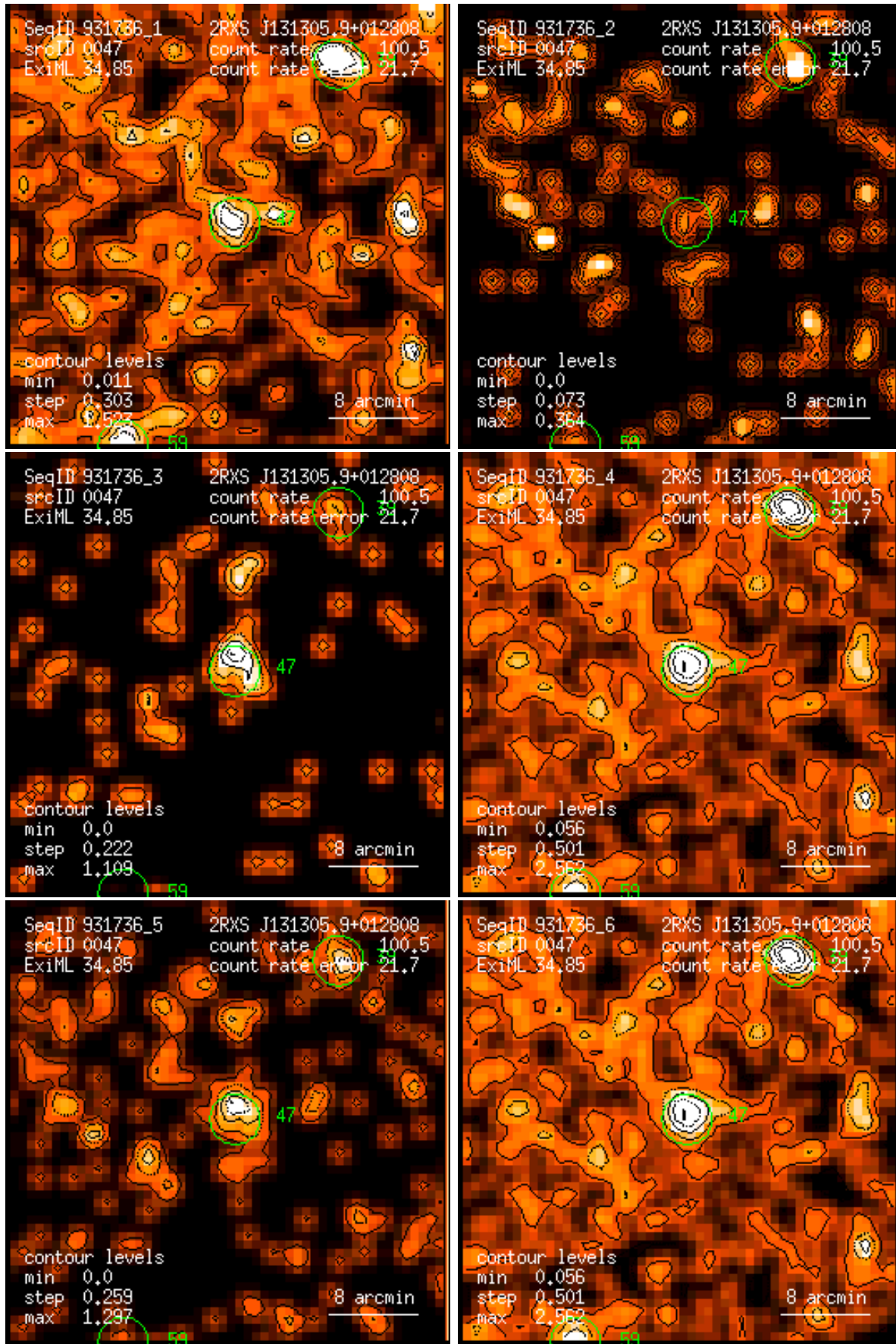
Figure 47: RASS 931736: detection 0047: band rate images, Gaussian filter: (1) PSPC channels 11 – 41, (2) 52 – 90, (3) 91 – 201, (4) 11 – 235, (5) 52 – 201, (6) 11 – 201. Broad band rates in counts/ks. Band rate contour levels in counts/ks/arcmin 2 .
