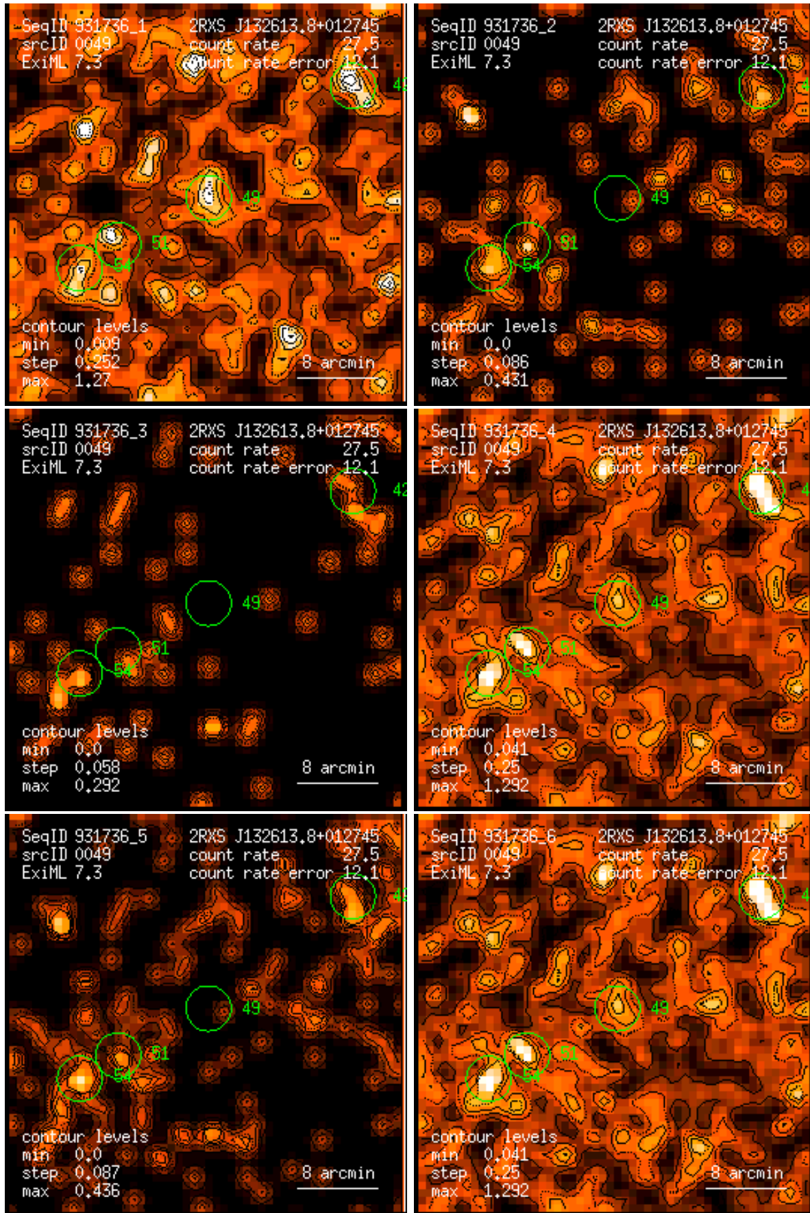
Figure 49: RASS 931736: detection 0049: band rate images, Gaussian filter: (1) PSPC channels 11 – 41, (2) 52 – 90, (3) 91 – 201, (4) 11 – 235, (5) 52 – 201, (6) 11 – 201. Broad band rates in counts/ks. Band rate contour levels in counts/ks/arcmin 2 .
