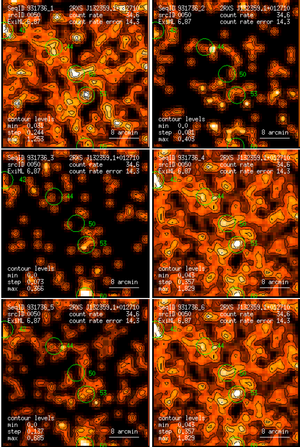
Figure 50: RASS 931736: detection 0050: band rate images, Gaussian filter: (1) PSPC channels 11 – 41, (2) 52 – 90, (3) 91 – 201, (4) 11 – 235, (5) 52 – 201, (6) 11 – 201. Broad band rates in counts/ks. Band rate contour levels in counts/ks/arcmin 2 .
