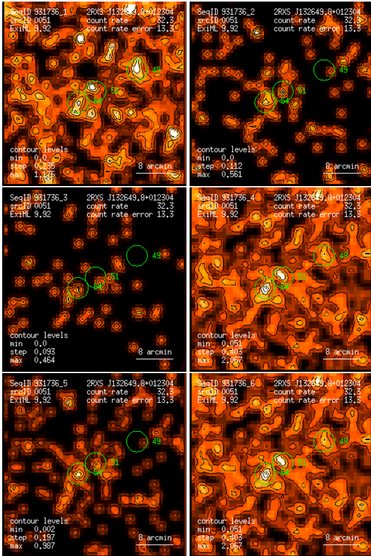
Figure 51: RASS 931736: detection 0051: band rate images, Gaussian filter: (1) PSPC channels 11 – 41, (2) 52 – 90, (3) 91 – 201, (4) 11 – 235, (5) 52 – 201, (6) 11 – 201. Broad band rates in counts/ks. Band rate contour levels in counts/ks/arcmin 2 .
