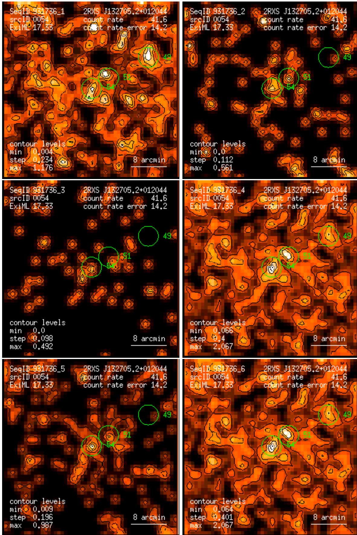
Figure 54: RASS 931736: detection 0054: band rate images, Gaussian filter: (1) PSPC channels 11 – 41, (2) 52 – 90, (3) 91 – 201, (4) 11 – 235, (5) 52 – 201, (6) 11 – 201. Broad band rates in counts/ks. Band rate contour levels in counts/ks/arcmin 2 .
