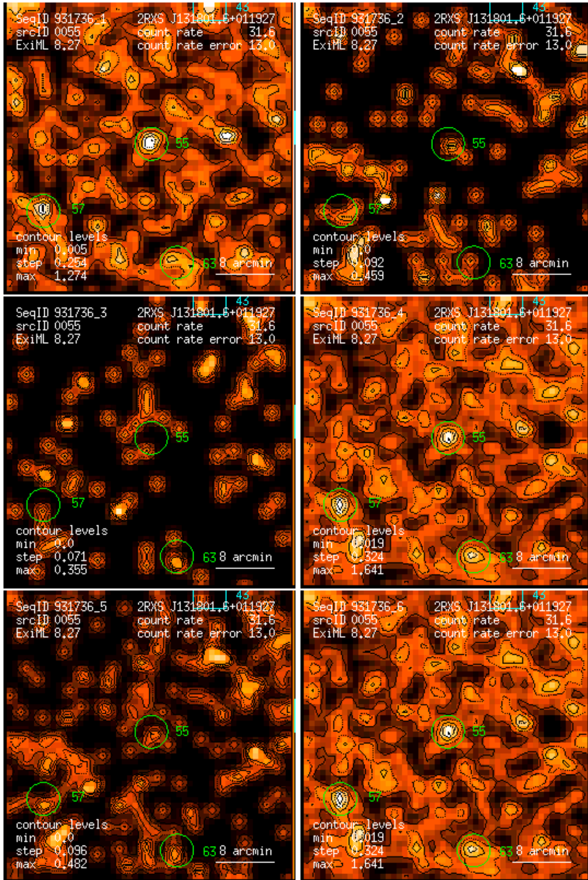
Figure 55: RASS 931736: detection 0055: band rate images, Gaussian filter: (1) PSPC channels 11 – 41, (2) 52 – 90, (3) 91 – 201, (4) 11 – 235, (5) 52 – 201, (6) 11 – 201. Broad band rates in counts/ks. Band rate contour levels in counts/ks/arcmin 2 .
