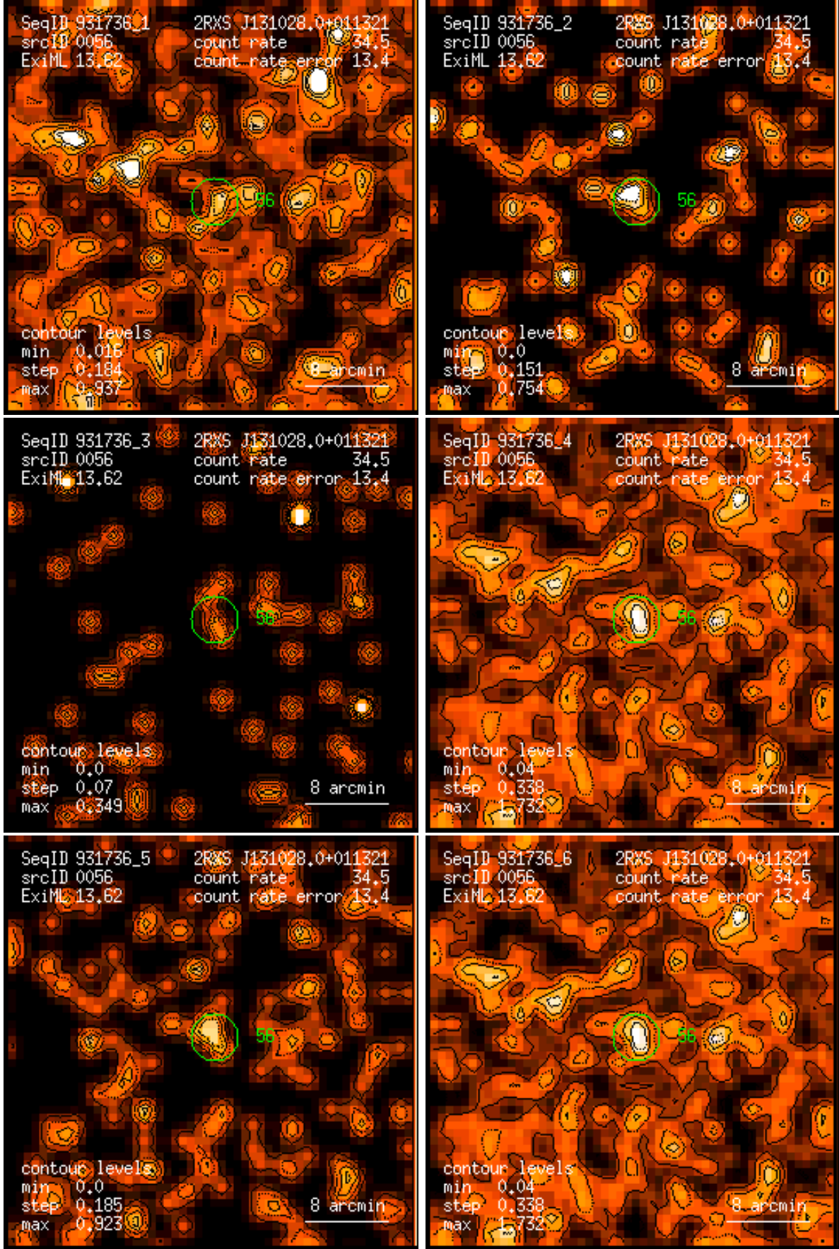
Figure 56: RASS 931736: detection 0056: band rate images, Gaussian filter: (1) PSPC channels 11 – 41, (2) 52 – 90, (3) 91 – 201, (4) 11 – 235, (5) 52 – 201, (6) 11 – 201. Broad band rates in counts/ks. Band rate contour levels in counts/ks/arcmin 2 .
