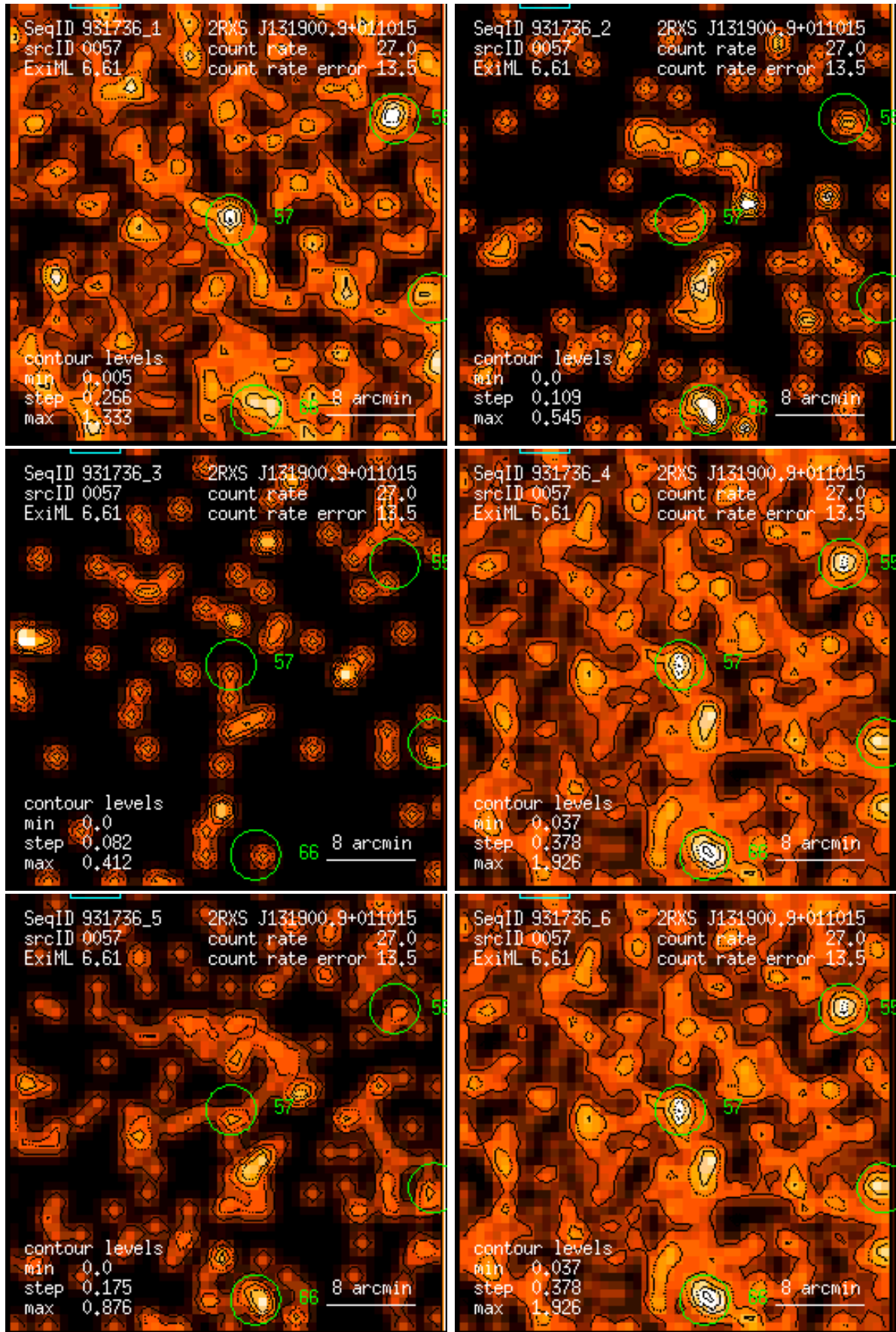
Figure 57: RASS 931736: detection 0057: band rate images, Gaussian filter: (1) PSPC channels 11 – 41, (2) 52 – 90, (3) 91 – 201, (4) 11 – 235, (5) 52 – 201, (6) 11 – 201. Broad band rates in counts/ks. Band rate contour levels in counts/ks/arcmin 2 .
