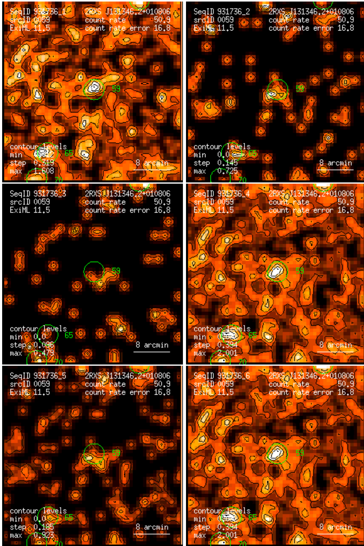
Figure 59: RASS 931736: detection 0059: band rate images, Gaussian filter: (1) PSPC channels 11 – 41, (2) 52 – 90, (3) 91 – 201, (4) 11 – 235, (5) 52 – 201, (6) 11 – 201. Broad band rates in counts/ks. Band rate contour levels in counts/ks/arcmin 2 .
