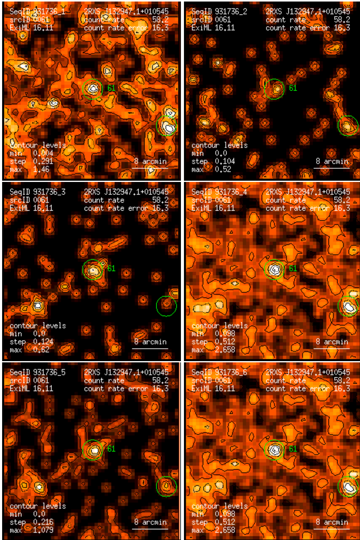
Figure 61: RASS 931736: detection 0061: band rate images, Gaussian filter: (1) PSPC channels 11 – 41, (2) 52 – 90, (3) 91 – 201, (4) 11 – 235, (5) 52 – 201, (6) 11 – 201. Broad band rates in counts/ks. Band rate contour levels in counts/ks/arcmin 2 .
