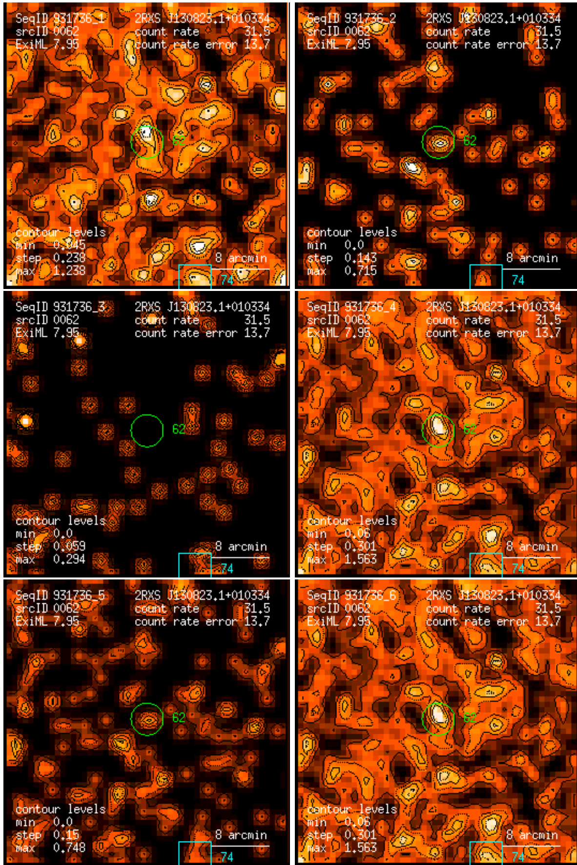
Figure 62: RASS 931736: detection 0062: band rate images, Gaussian filter: (1) PSPC channels 11 – 41, (2) 52 – 90, (3) 91 – 201, (4) 11 – 235, (5) 52 – 201, (6) 11 – 201. Broad band rates in counts/ks. Band rate contour levels in counts/ks/arcmin 2 .
