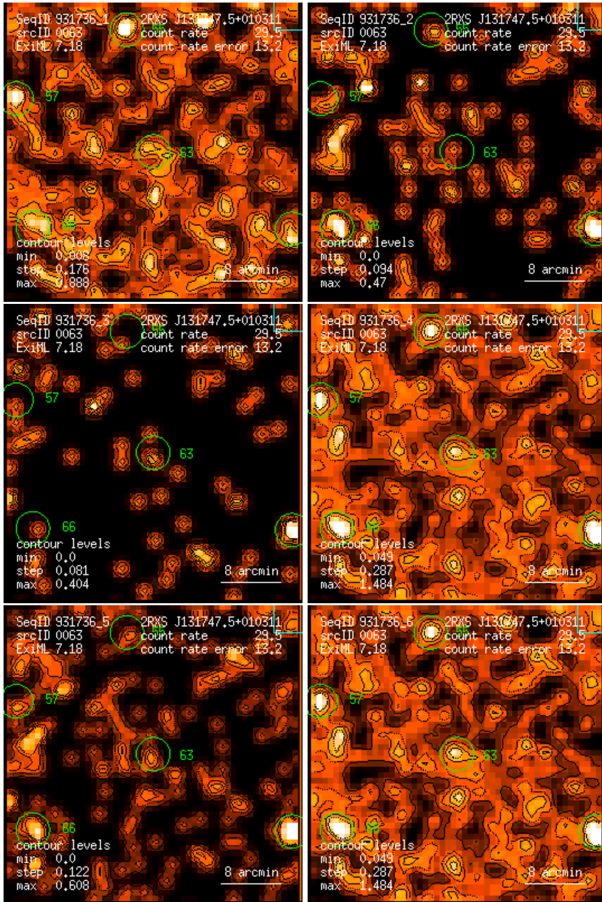
Figure 63: RASS 931736: detection 0063: band rate images, Gaussian filter: (1) PSPC channels 11 – 41, (2) 52 – 90, (3) 91 – 201, (4) 11 – 235, (5) 52 – 201, (6) 11 – 201. Broad band rates in counts/ks. Band rate contour levels in counts/ks/arcmin 2 .
