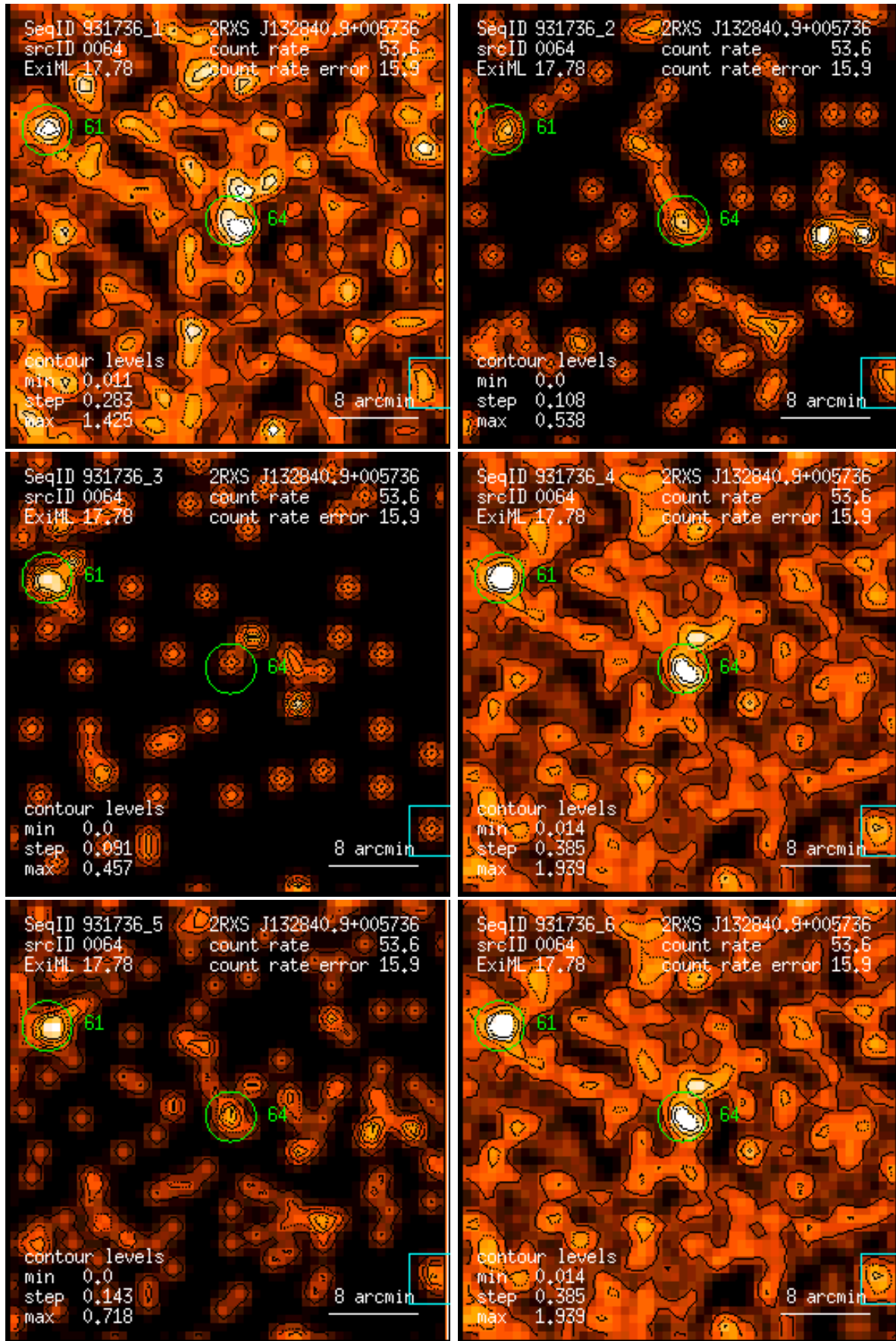
Figure 64: RASS 931736: detection 0064: band rate images, Gaussian filter: (1) PSPC channels 11 – 41, (2) 52 – 90, (3) 91 – 201, (4) 11 – 235, (5) 52 – 201, (6) 11 – 201. Broad band rates in counts/ks. Band rate contour levels in counts/ks/arcmin 2 .
