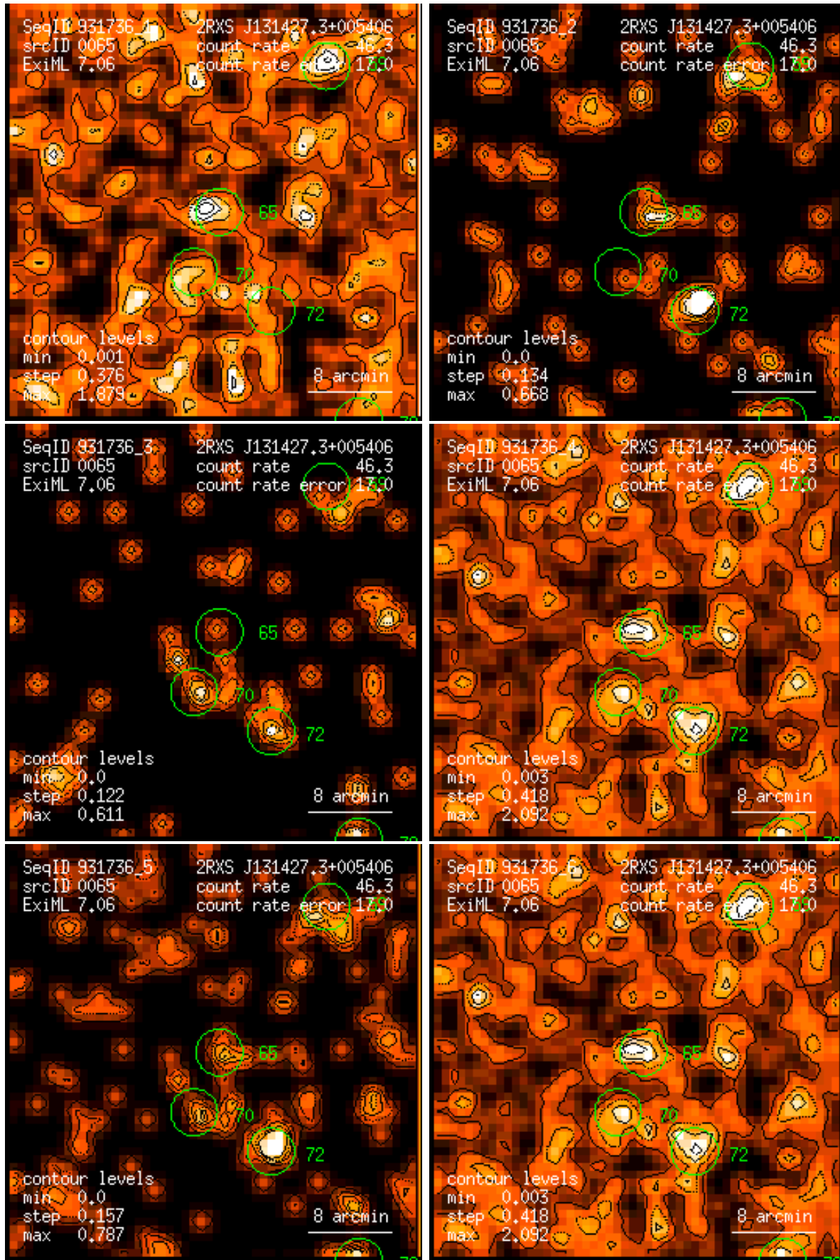
Figure 65: RASS 931736: detection 0065: band rate images, Gaussian filter: (1) PSPC channels 11 – 41, (2) 52 – 90, (3) 91 – 201, (4) 11 – 235, (5) 52 – 201, (6) 11 – 201. Broad band rates in counts/ks. Band rate contour levels in counts/ks/arcmin 2 .
