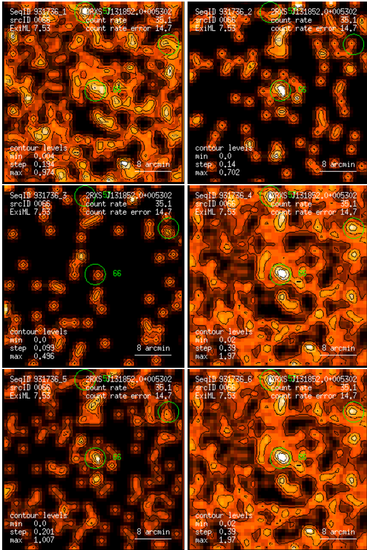
Figure 66: RASS 931736: detection 0066: band rate images, Gaussian filter: (1) PSPC channels 11 – 41, (2) 52 – 90, (3) 91 – 201, (4) 11 – 235, (5) 52 – 201, (6) 11 – 201. Broad band rates in counts/ks. Band rate contour levels in counts/ks/arcmin 2 .
