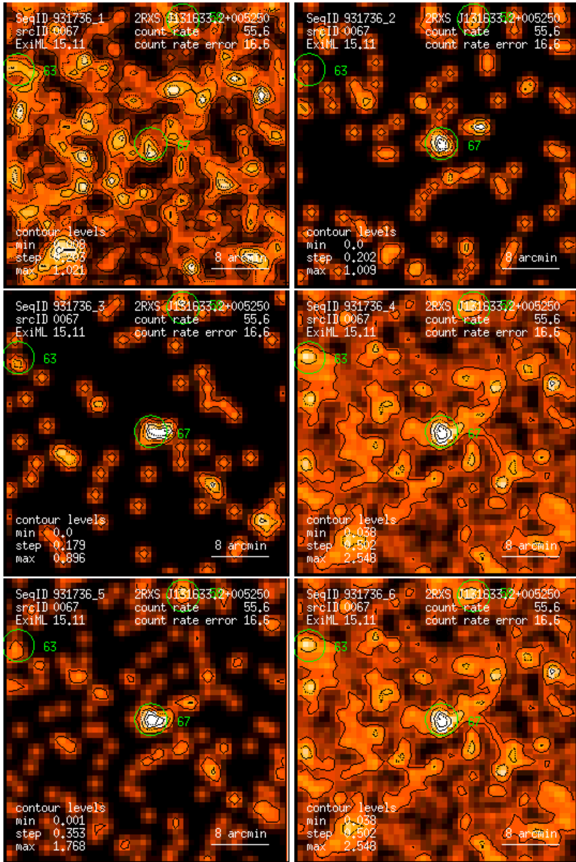
Figure 67: RASS 931736: detection 0067: band rate images, Gaussian filter: (1) PSPC channels 11 – 41, (2) 52 – 90, (3) 91 – 201, (4) 11 – 235, (5) 52 – 201, (6) 11 – 201. Broad band rates in counts/ks. Band rate contour levels in counts/ks/arcmin 2 .
