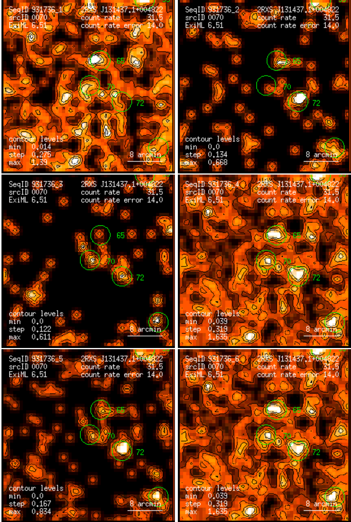
Figure 70: RASS 931736: detection 0070: band rate images, Gaussian filter: (1) PSPC channels 11 – 41, (2) 52 – 90, (3) 91 – 201, (4) 11 – 235, (5) 52 – 201, (6) 11 – 201. Broad band rates in counts/ks. Band rate contour levels in counts/ks/arcmin 2 .
